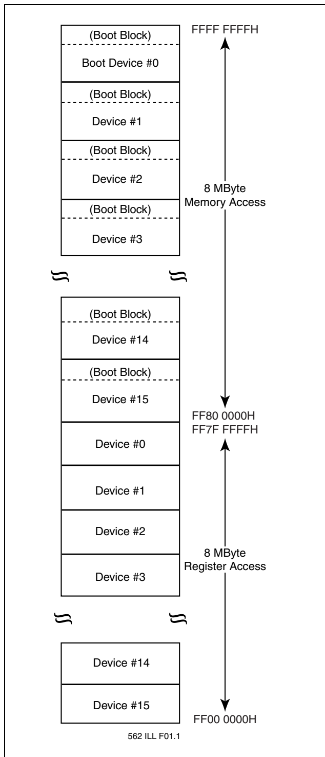
FIGURE 4: BOOT CONFIGURATION FROM THE TOP OF THE 4 GByte SYSTEM MEMORY MAP
