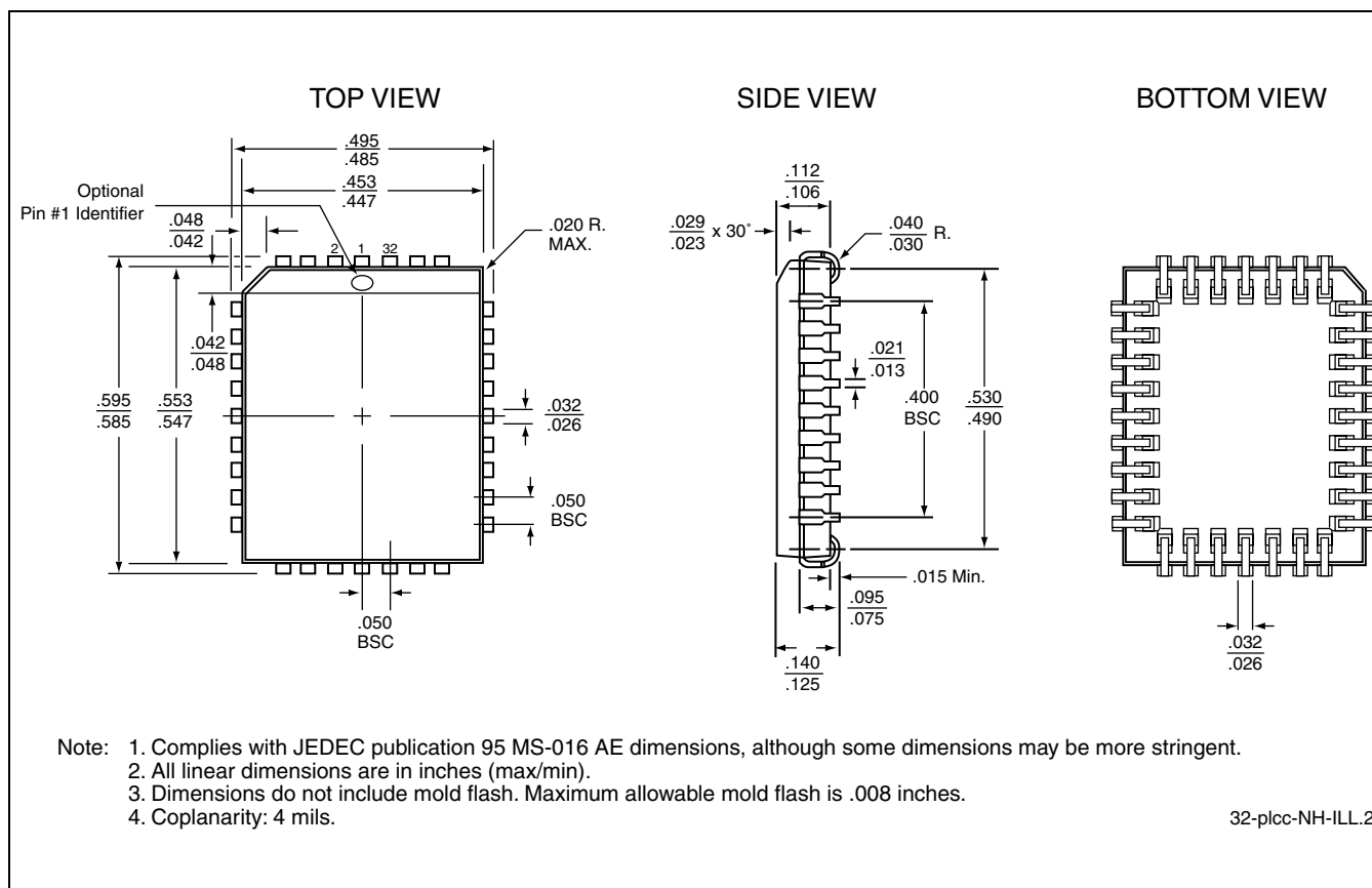
32-LEAD PLASTIC LEAD CHIP CARRIER (PLCC) SST PACKAGE CODE: NH
