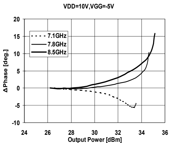
AMPM vs OUTPUT POWER
