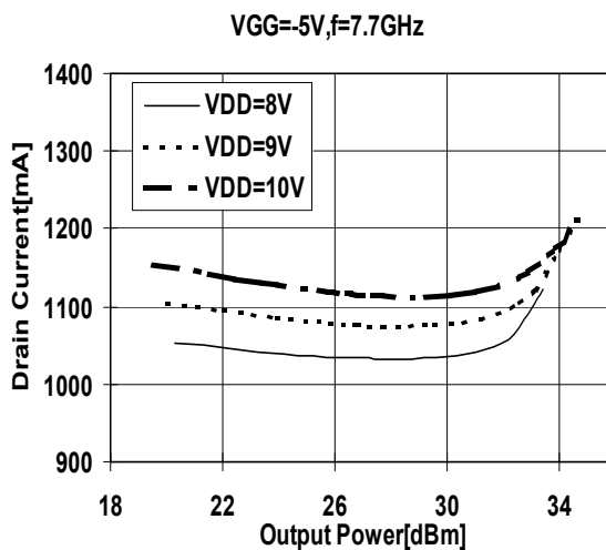
DRAIN CURRENT vs OUTPUT POWER
