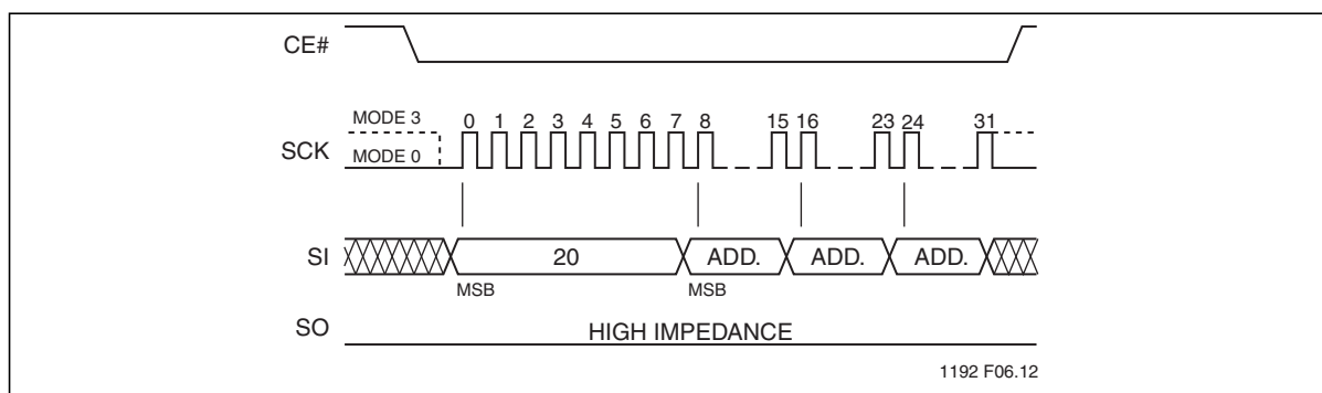
Figure 7: Sector-Erase Sequence
