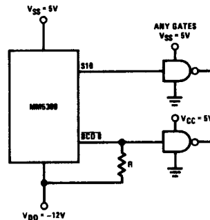
MOS to TTL Interface
