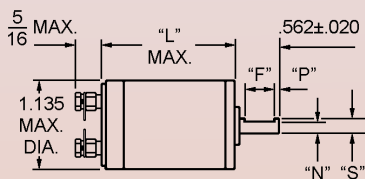
Figure 10 Instrument/Industrial Configuration
