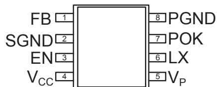
MSOP-8
