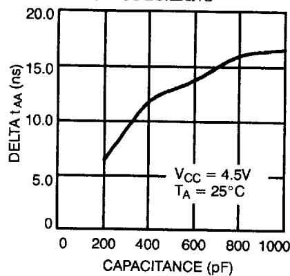
TYPICAL ACCESS TIME CHANGE vs. OUTPUT LOADING
