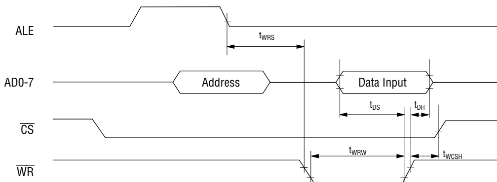
Write Timing
