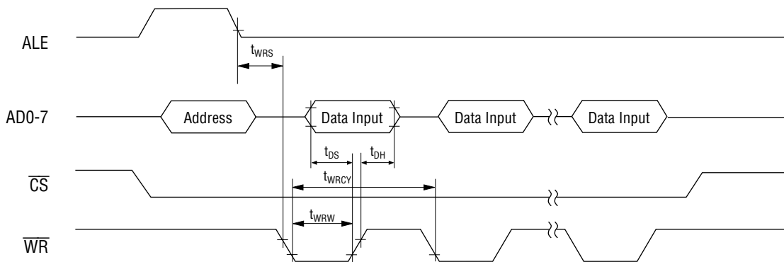
Write Timing
