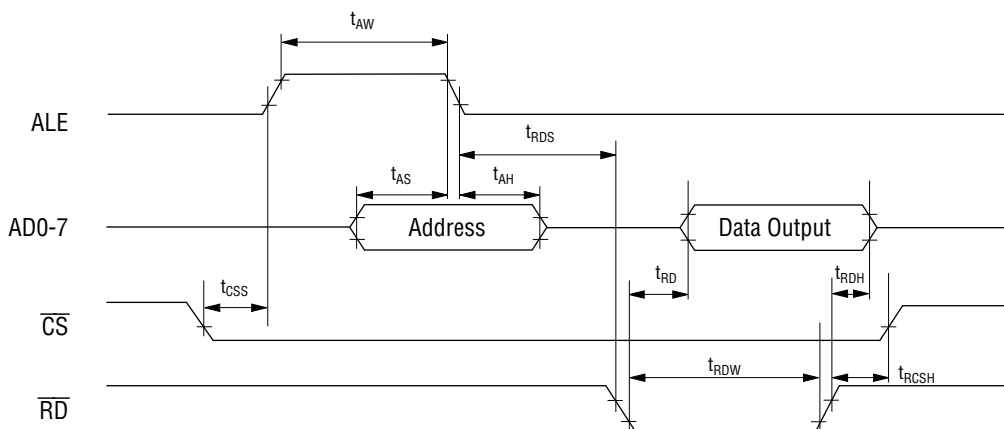
Read Timing
