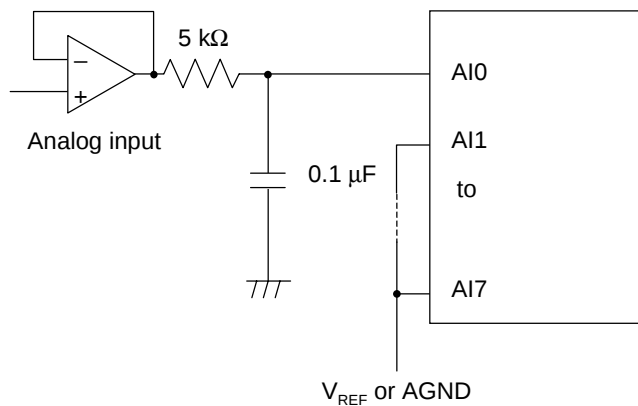
Measurement Circuit 2
