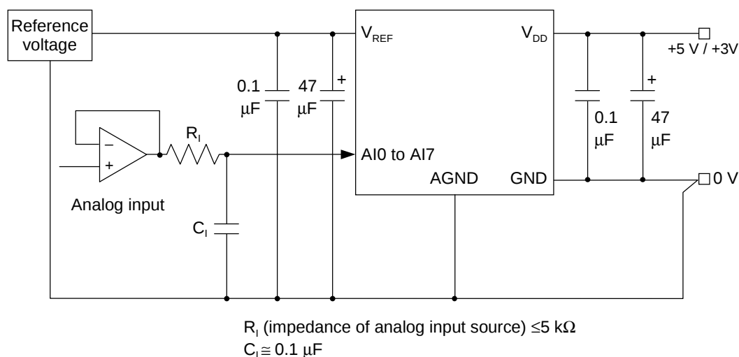
Measurement Circuit 1
