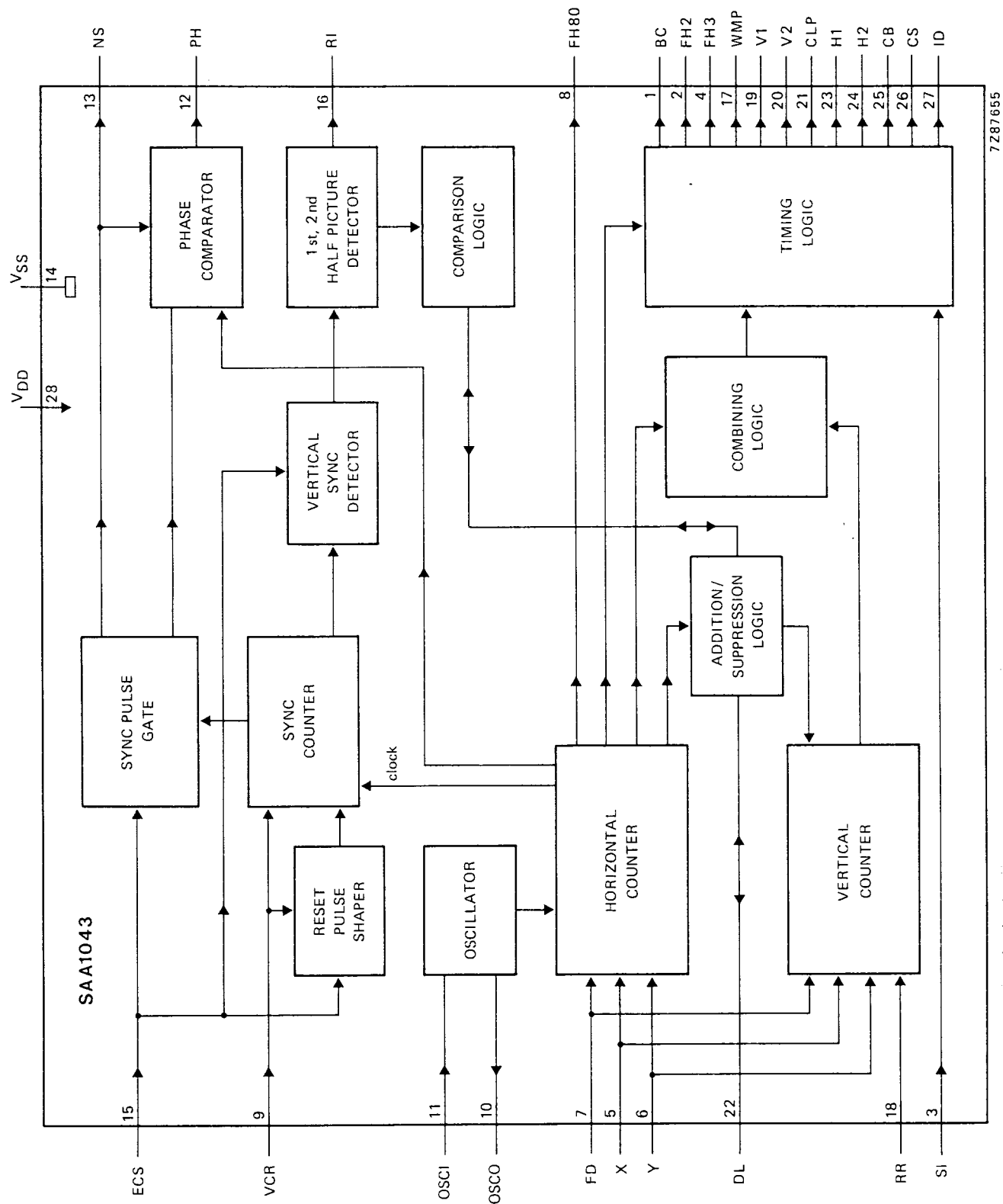
Fig. 1 Block diagram.
