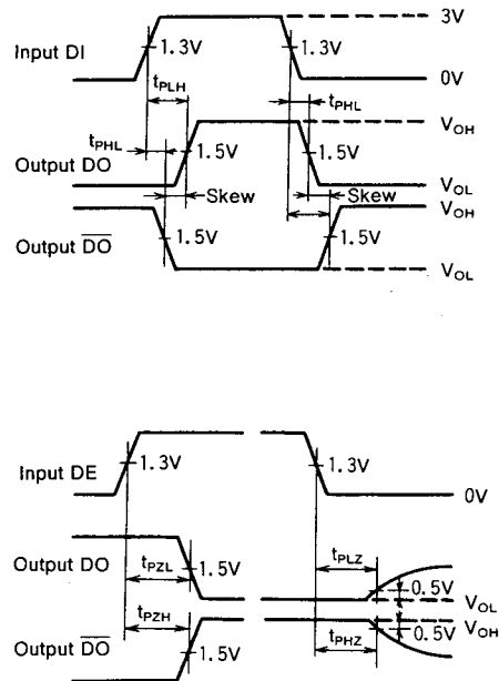
Driver Section
