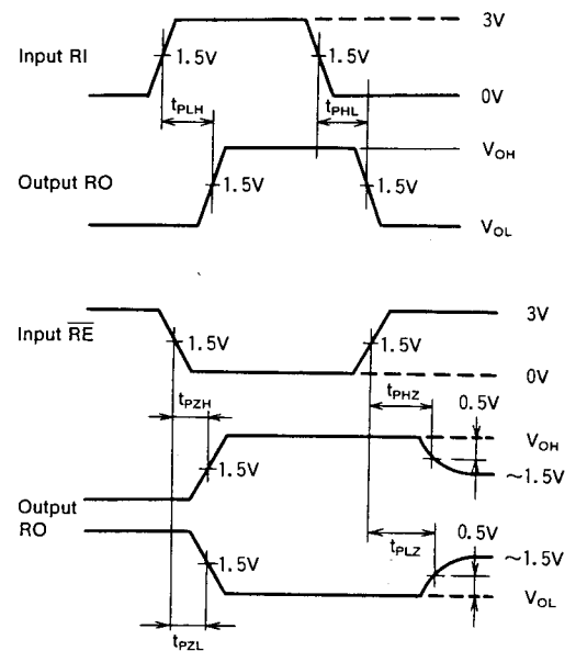
Receiver Section
