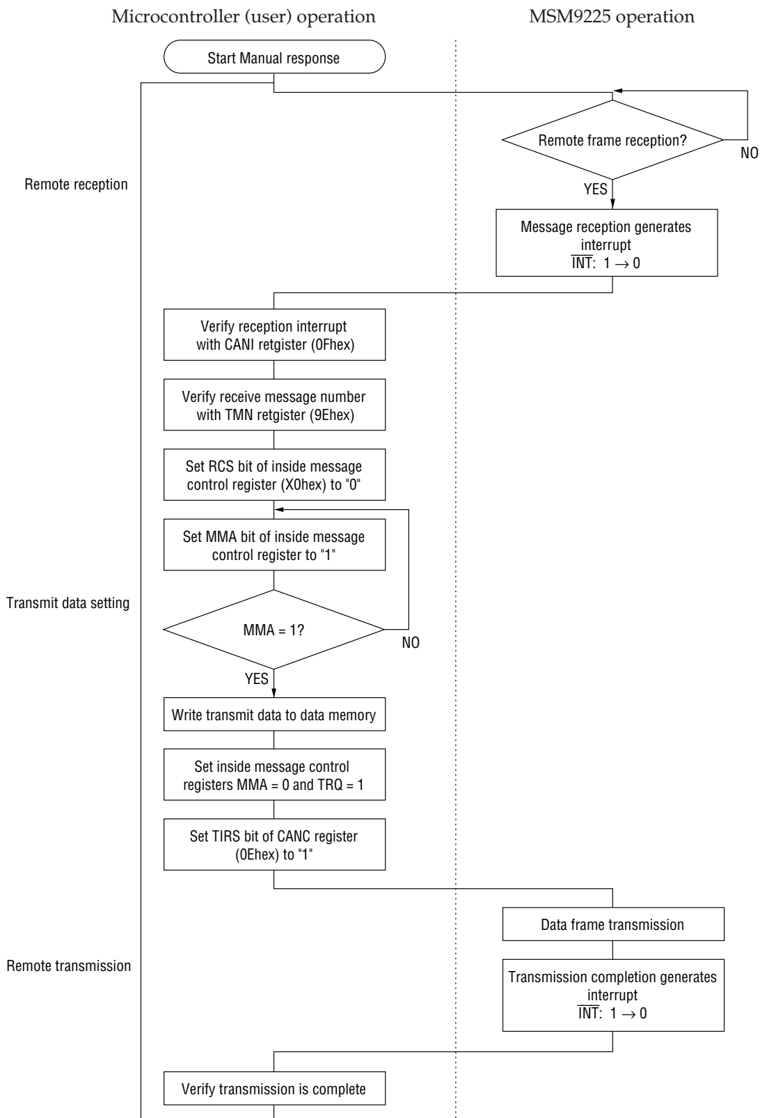
Figure: Manual Response Operation Flow Chart
