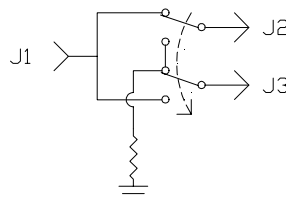
Switch Schematic
