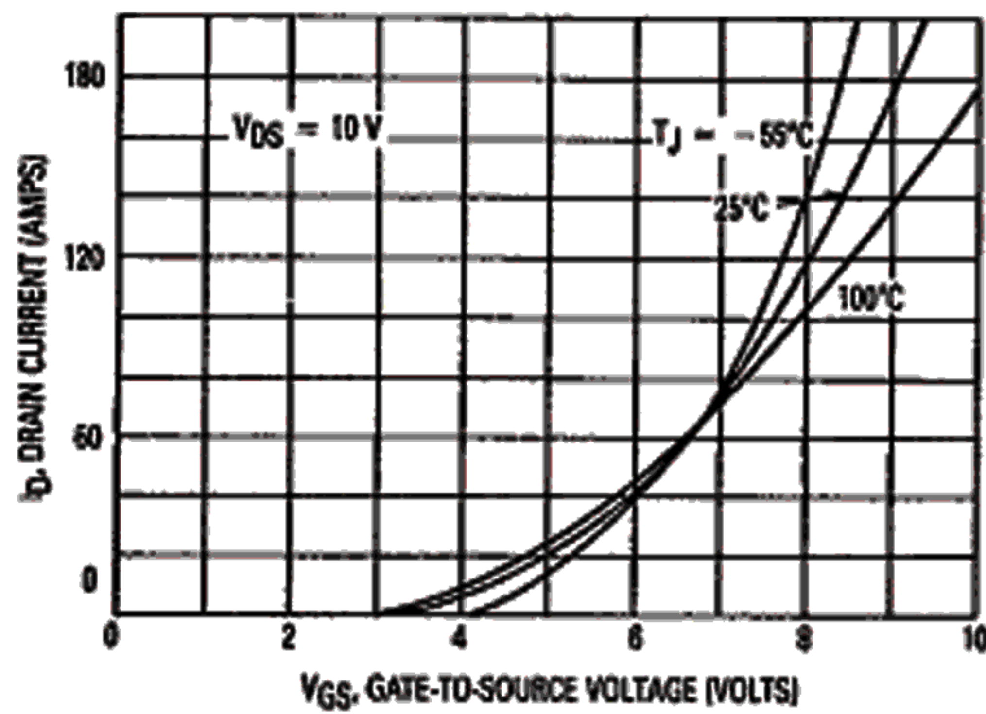
Figure 3. Transfer Characteristics
