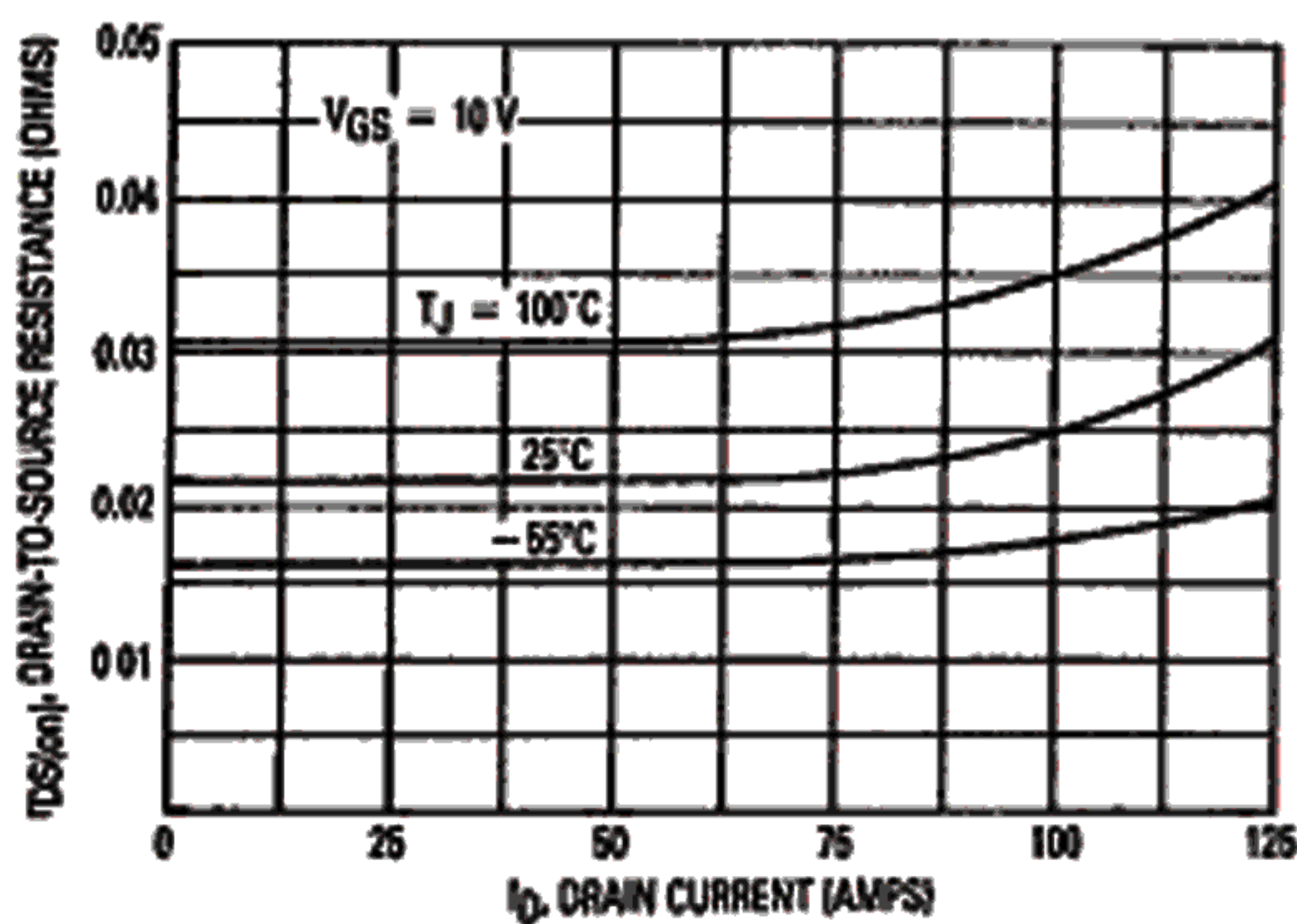
Figure 5. On-Resistance versus Drain Current
