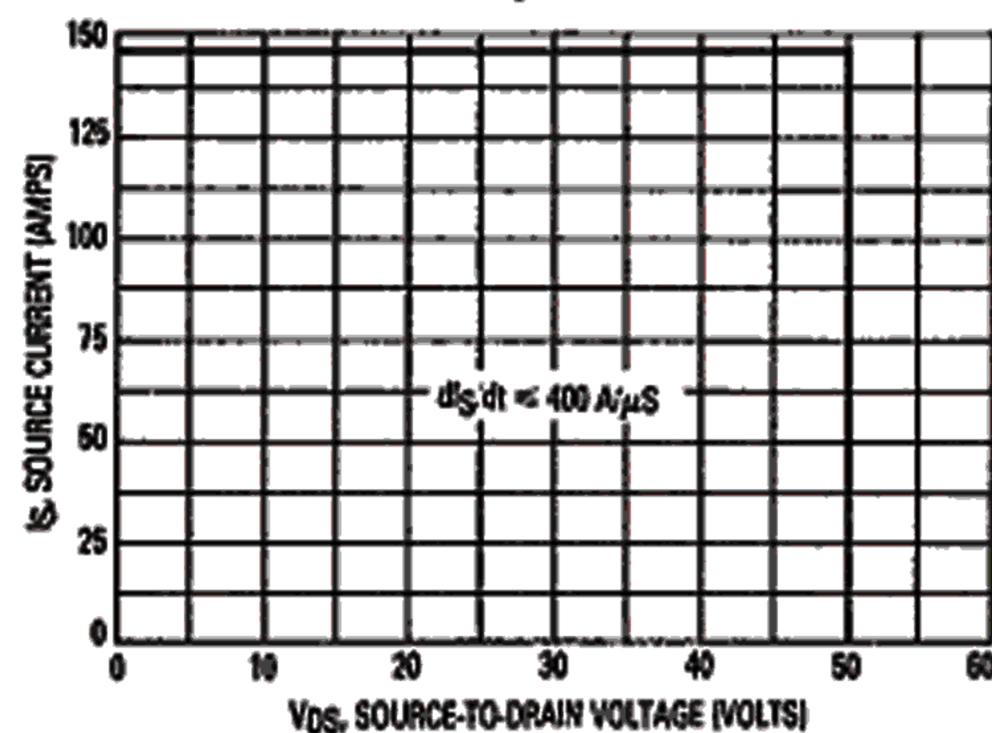
Figure 12. Commutating Safe Operating Area (CSOA)
