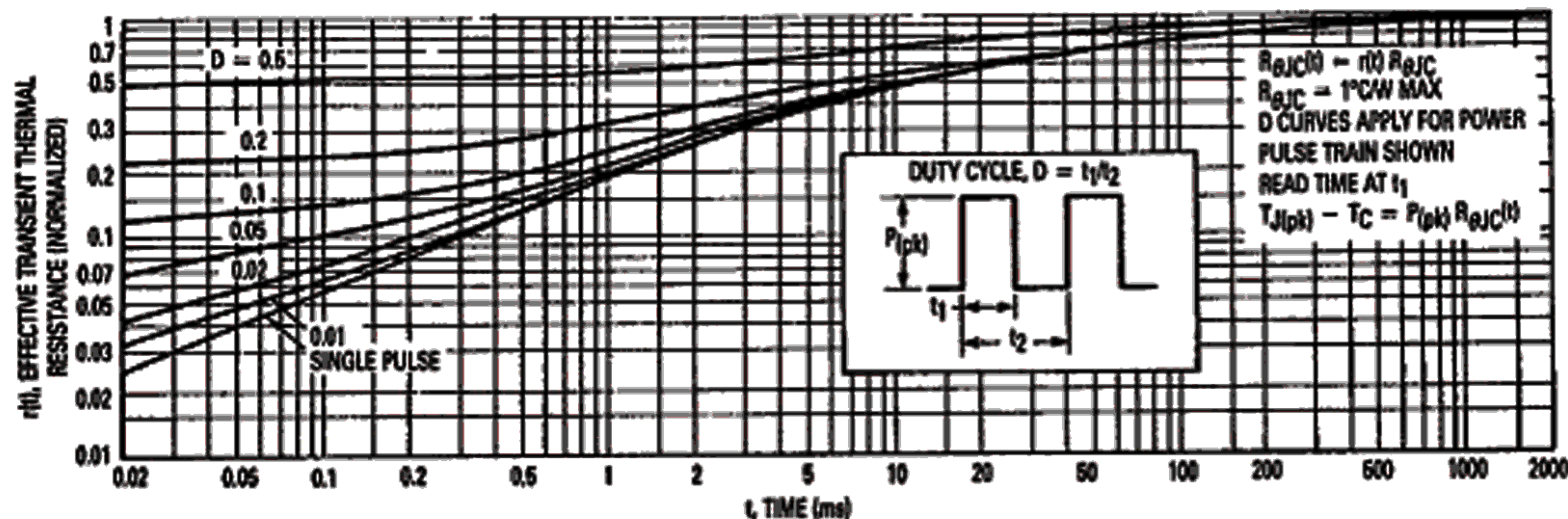
Figure 10. Thermal Response
