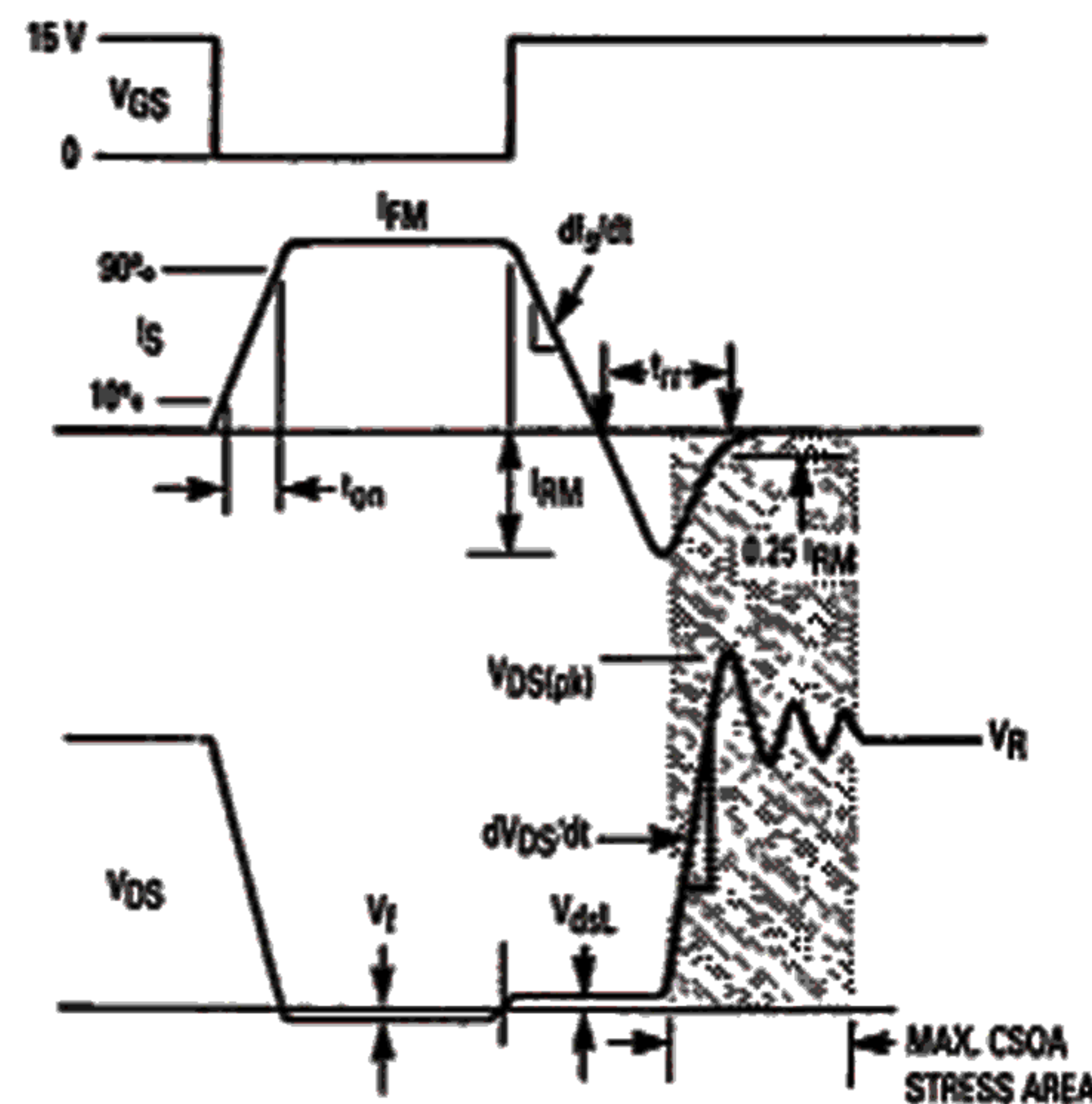
Figure 11. Commutating Waveforms
