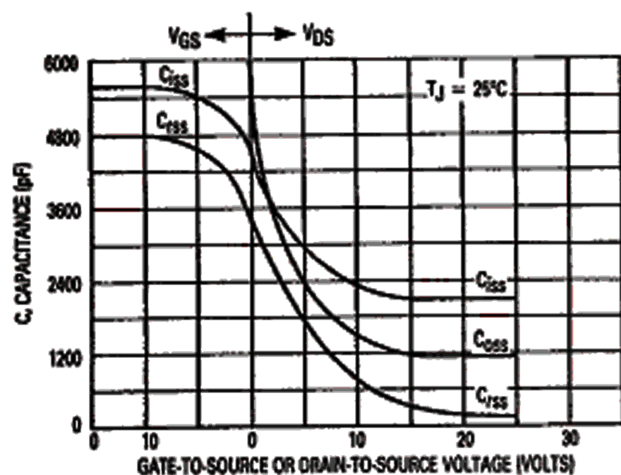
Figure 16. Capacitance Variation
