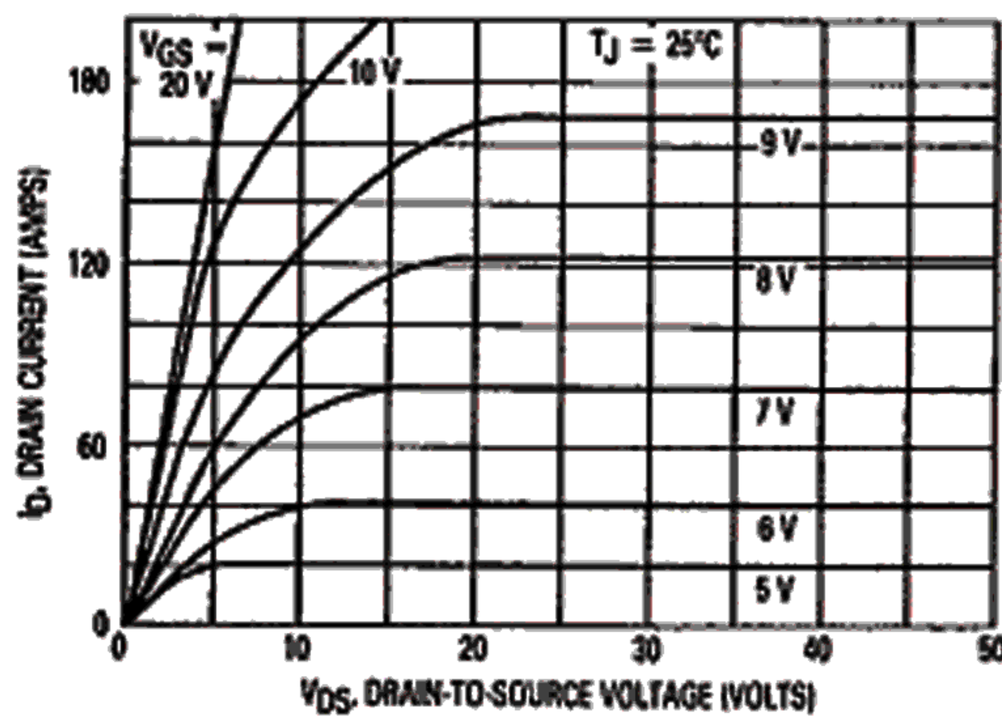
Figure 1. On-Region Characteristics
