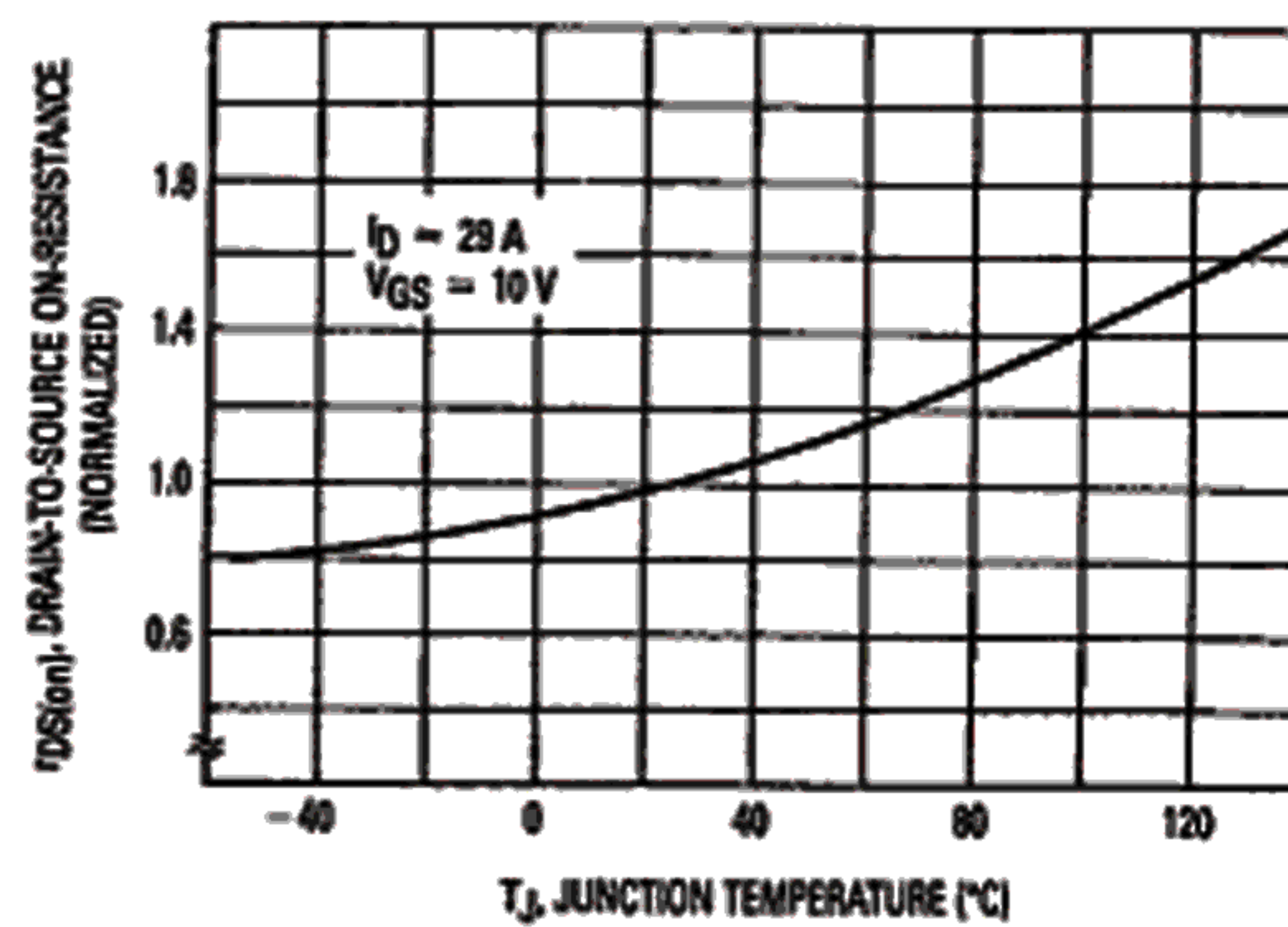
Figure 6. On-Resistance Variation With Temperature
