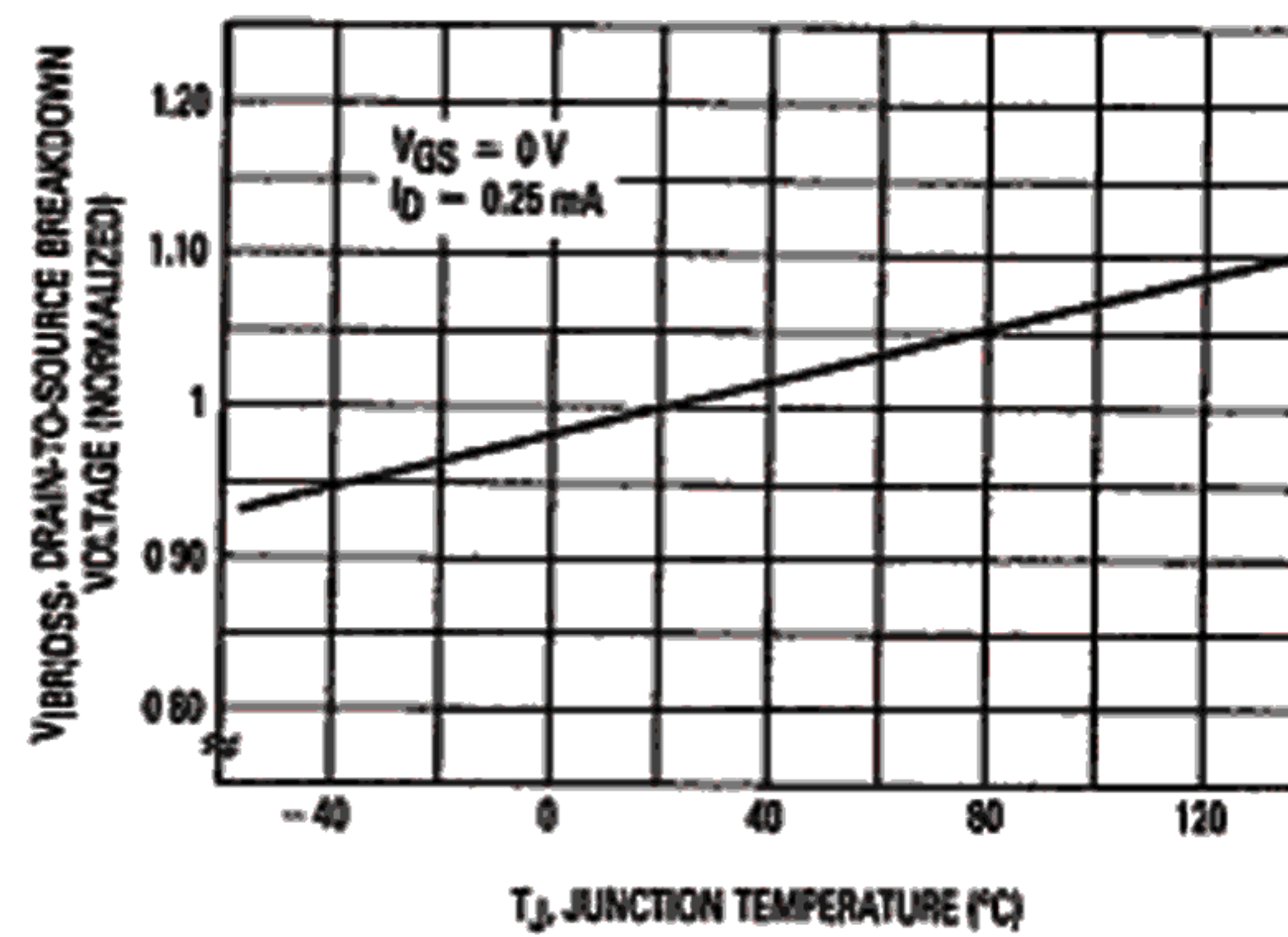
Figure 4. Breakdown Voltage Variation With Temperature
