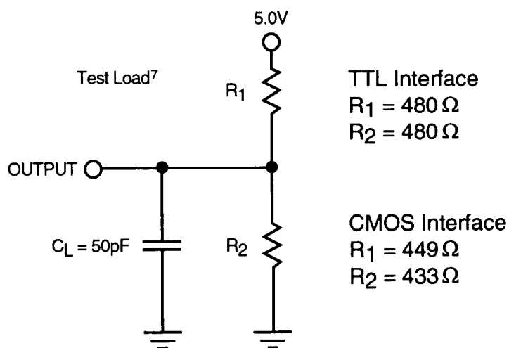
Figure 31: PEEL153 AC Test Loads
