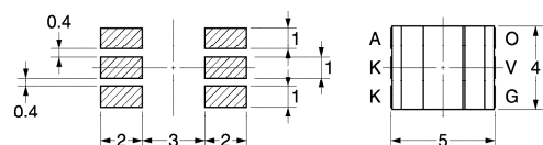
Recommended soldering patterns
