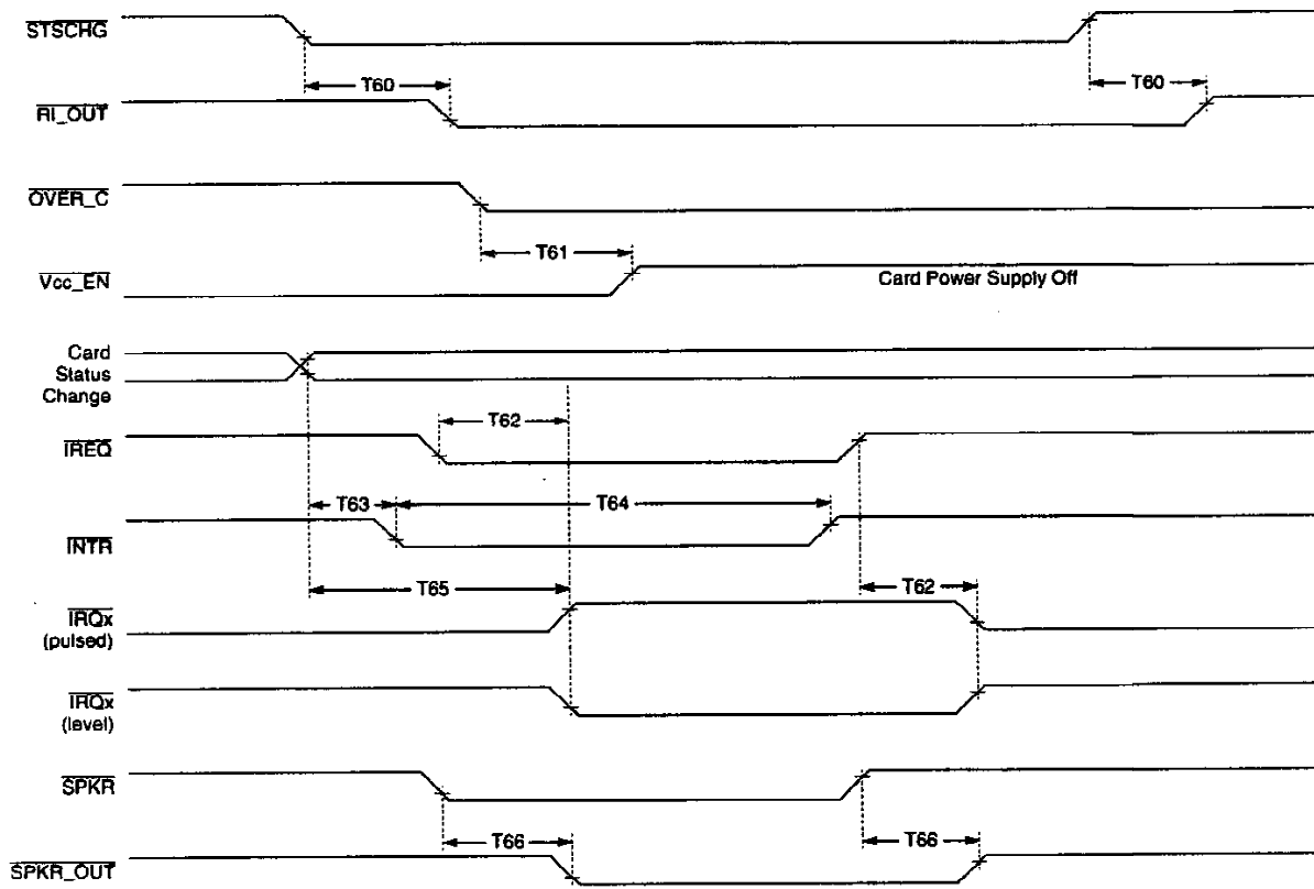
Figure 7. SPKR, STCHG, \overline{OVER\_C} and Interrupt Timing
