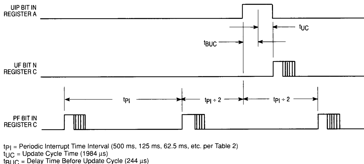
Figure 5.2. Update Ended and Periodic Relationships
