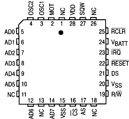
MCCS146818BFN CASE 776 PQCC
