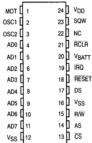
MCCS146818BP MCCS156818BP CASE 709 PLASTIC DIP
