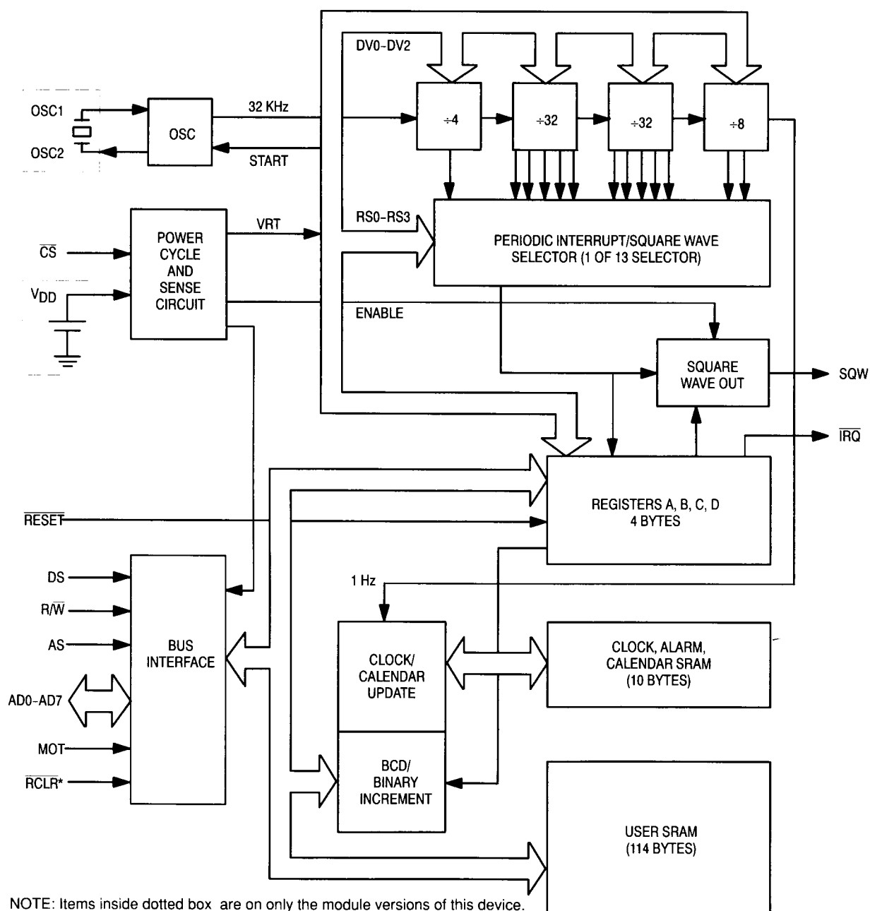
Figure 1.1. Block Diagram
