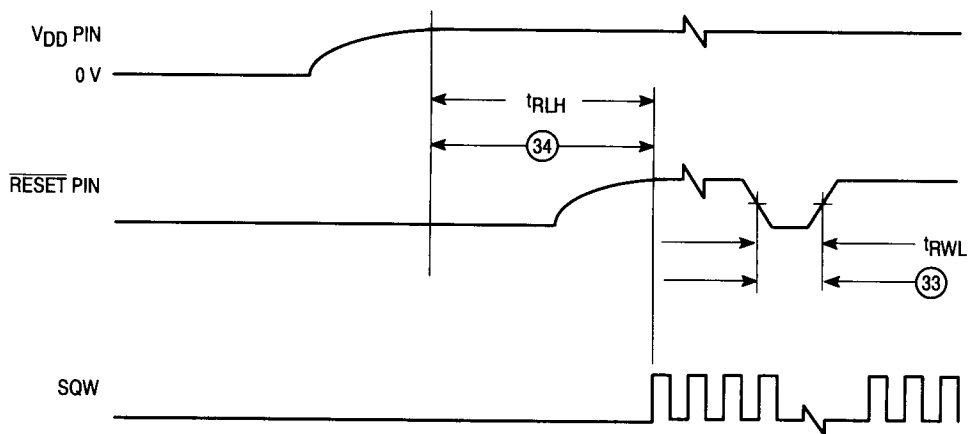
Figure 2.5. Power-Up Timing
