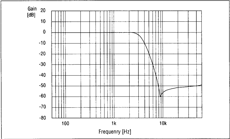
LPF Frequency Characteristics ( f_{sam}=8.0\text{kHz} )
