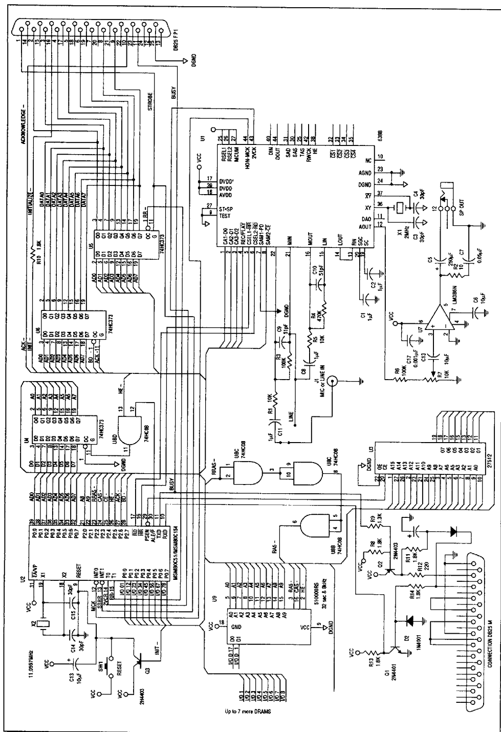
MSM6388 with 80C154 and DRAMS
