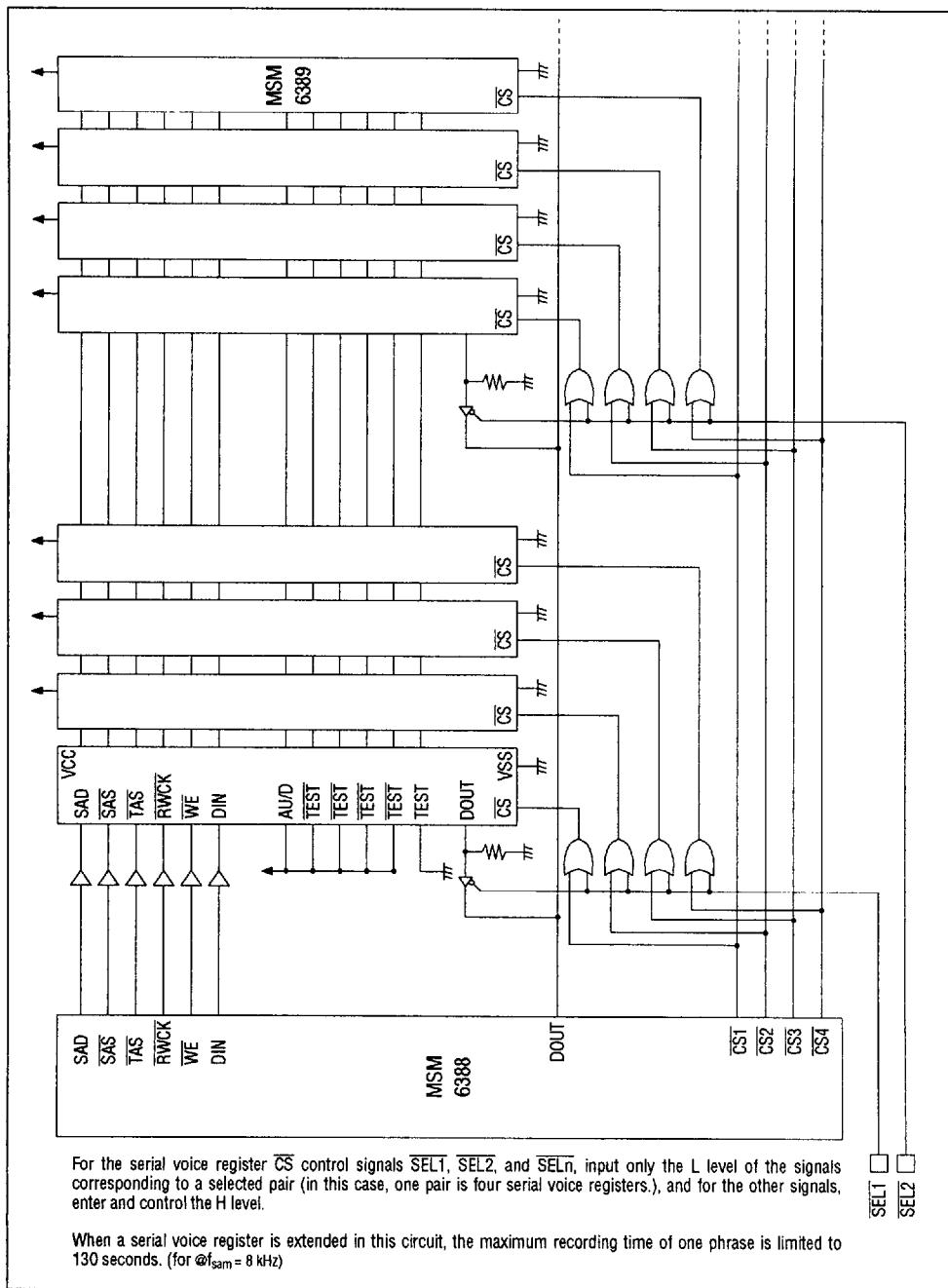
Circuit Diagram 5
