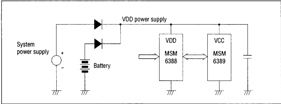
Figure: Example of Battery Backup Circuits of MSM6388 and MSM6389
