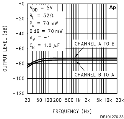
Channel Separation
