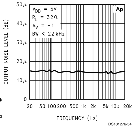
Noise Floor
