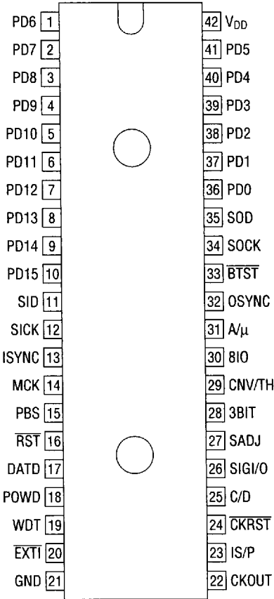
42-Pin Plastic DIP MSM6981-01RS
