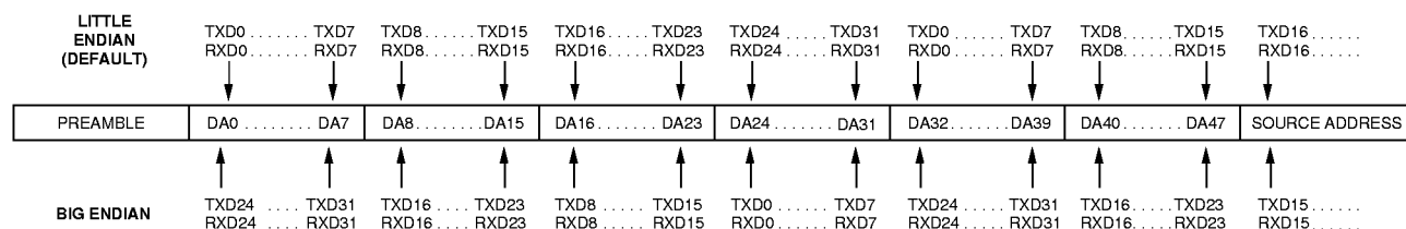
Figure 4. Little Endian vs. Big Endian Format
