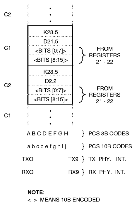
Figure 6. AutoNegotiation Data Format
