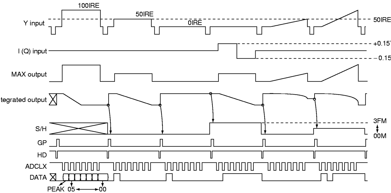
Timing Chart 2
