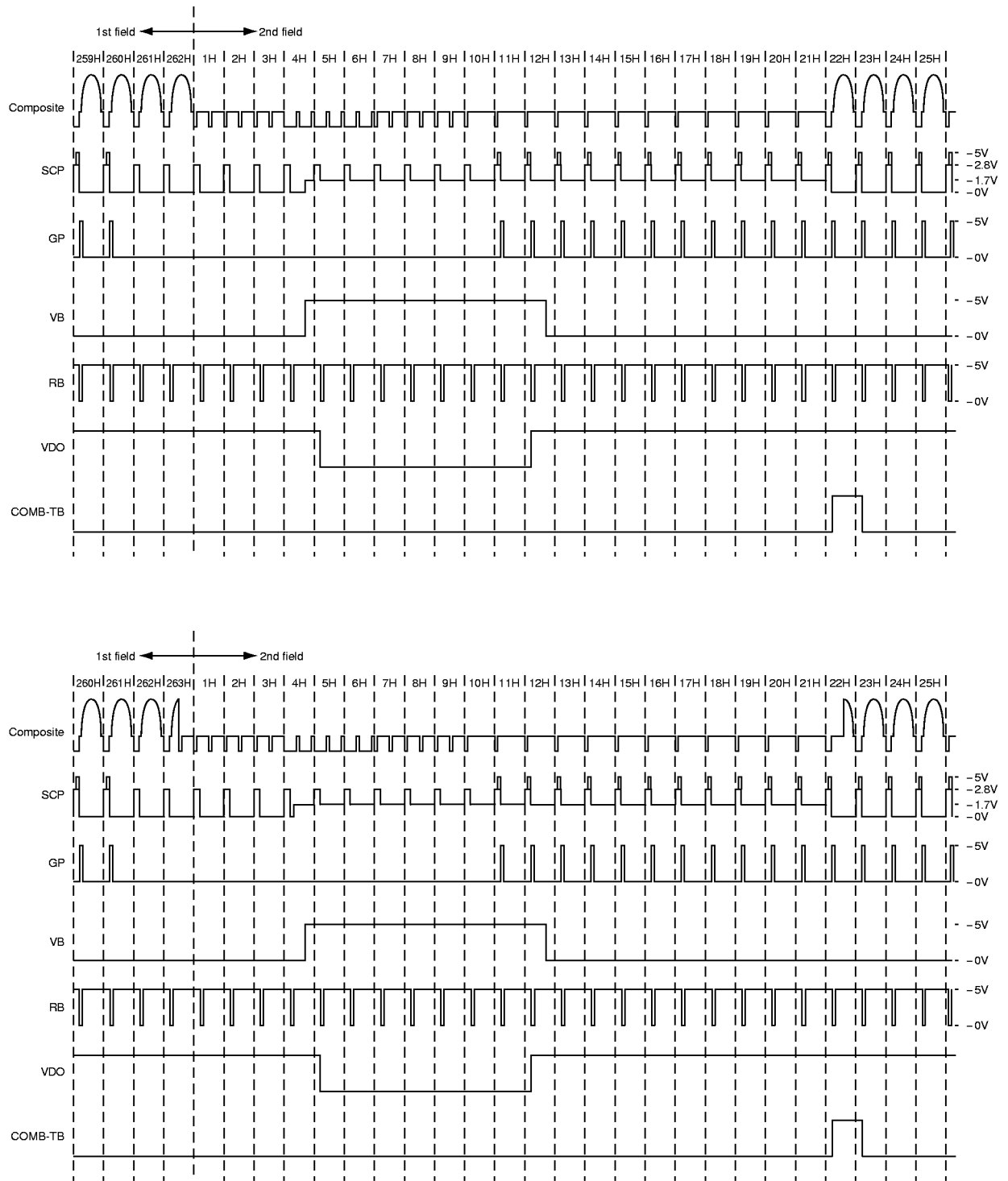
Timing Chart 1
