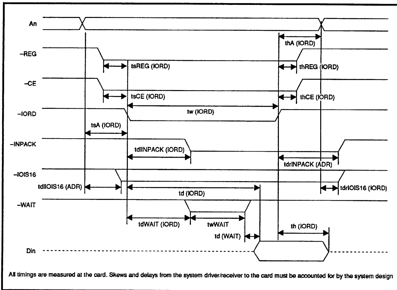
FIGURE 17: I/O Output Timing Specification (READ)
