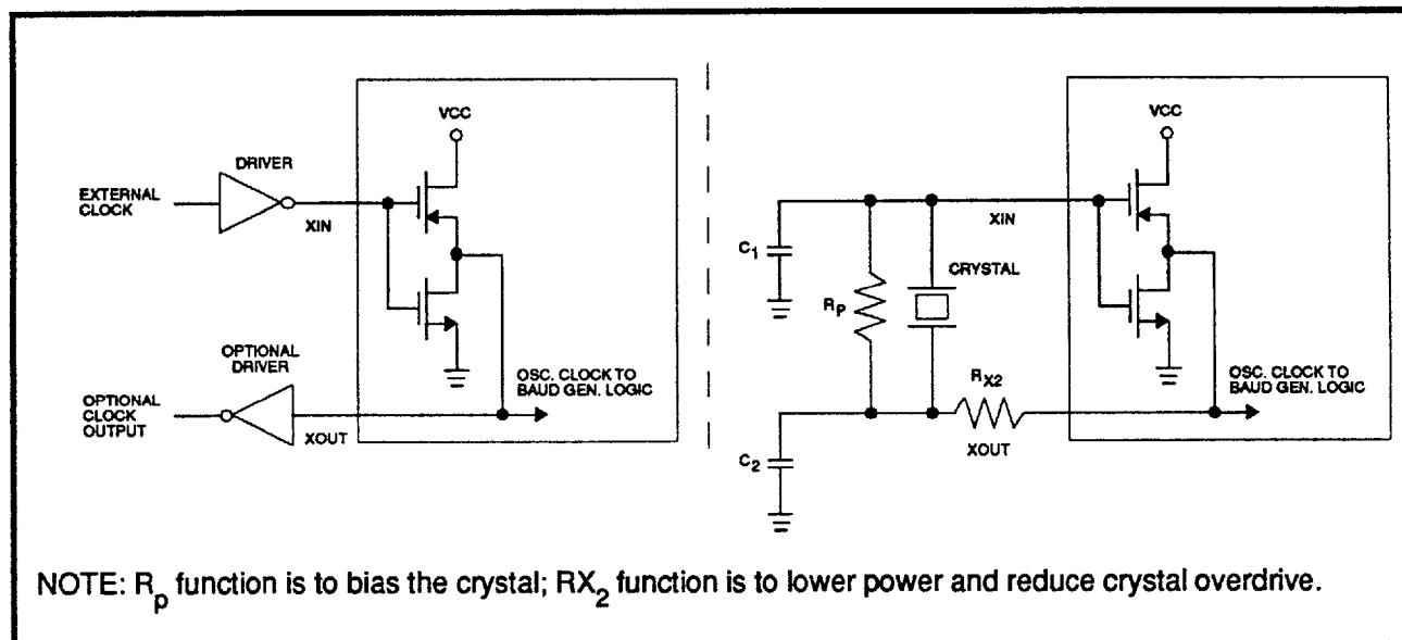
FIGURE 1: Typical Clock Circuits
