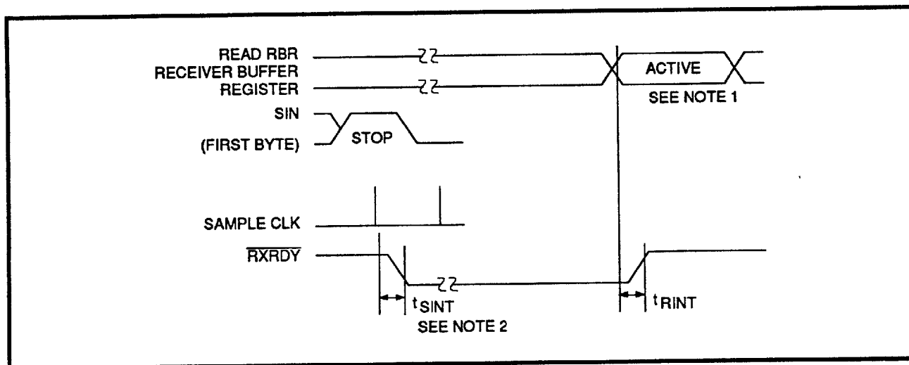
FIGURE 14: Receiver Ready (Pin 29) FCR D0 = 0 or FCR D0 = 1 and FCR D3 = 0 (Mode 0)
