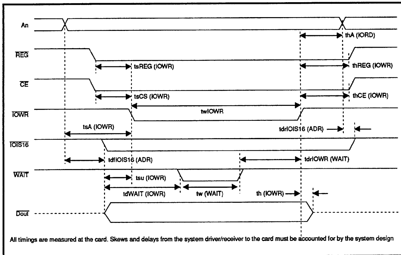
FIGURE 16: I/O Output Timing Specification (WRITE)
