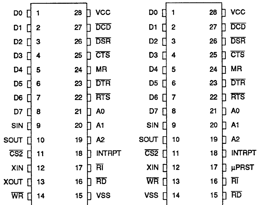
SSI 73M2550 UART 28-Pin DIP
