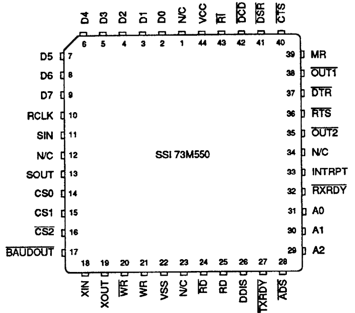
SSI 73M550 44-Pin PLCC
