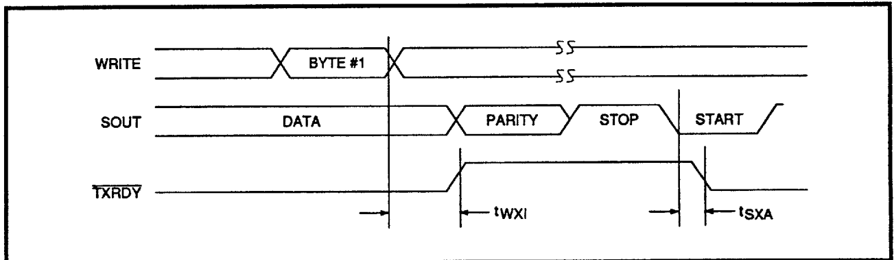
FIGURE 7: Transmitter Ready (Pin 24) FCR D0 = 0 or FCR D0 = 1 and FCR D3 = 0 (Mode 0)
