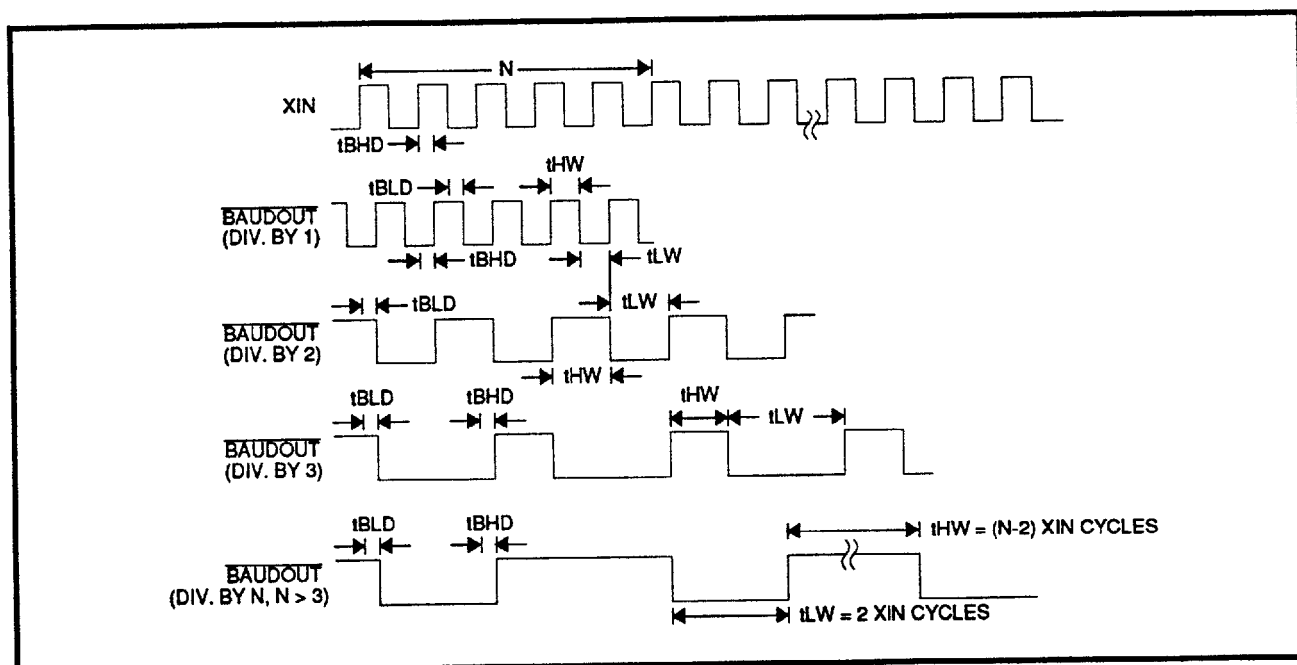
FIGURE 10: BAUDOUT Timing
