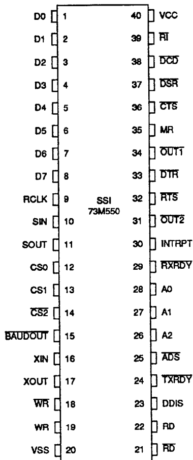
SSI 73M550 40-Pin DIP
