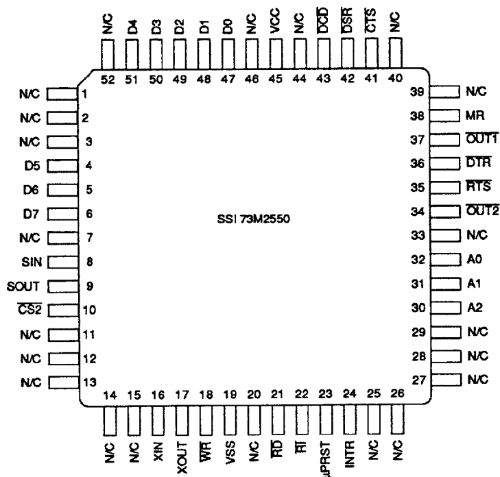
SSI 73M2550 52-Lead QFP
