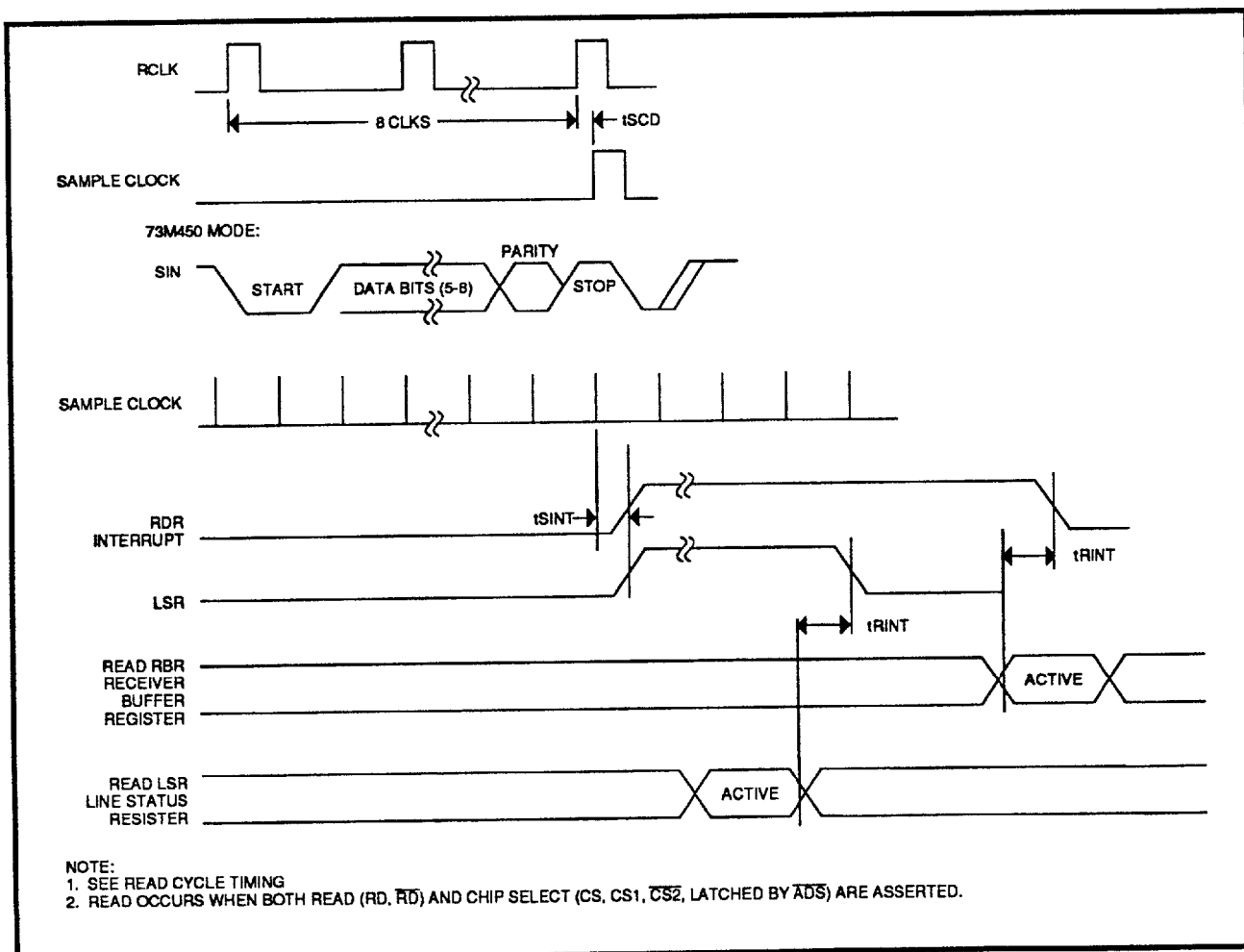
FIGURE 11: Receiver Timing
