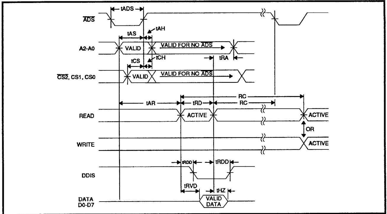
FIGURE 4: Read Cycle Timing
