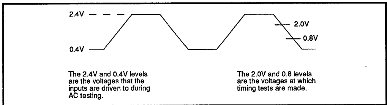
FIGURE 3: AC Test Points*
