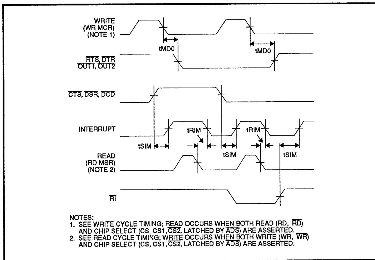
FIGURE 9: Modem Controls Timing
