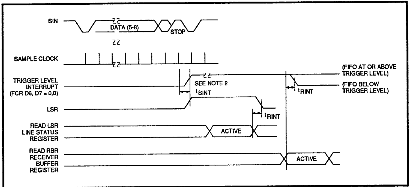
FIGURE 12: RCVr FIFO First Byte (This sets RBR)
