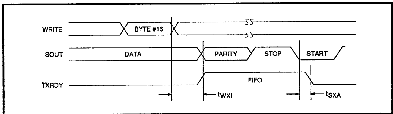
FIGURE 8: Transmitter Ready (Pin 24) FCR D0 = 1 and FCR D3 = 1 (Mode 1)
