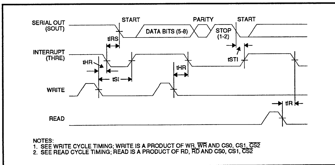
FIGURE 6: Transmitter Timing
