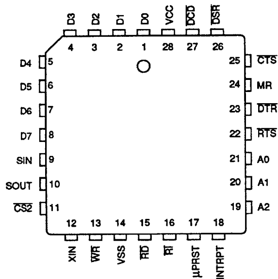
SSI 73M2550 UART 28-Pin PLCC
