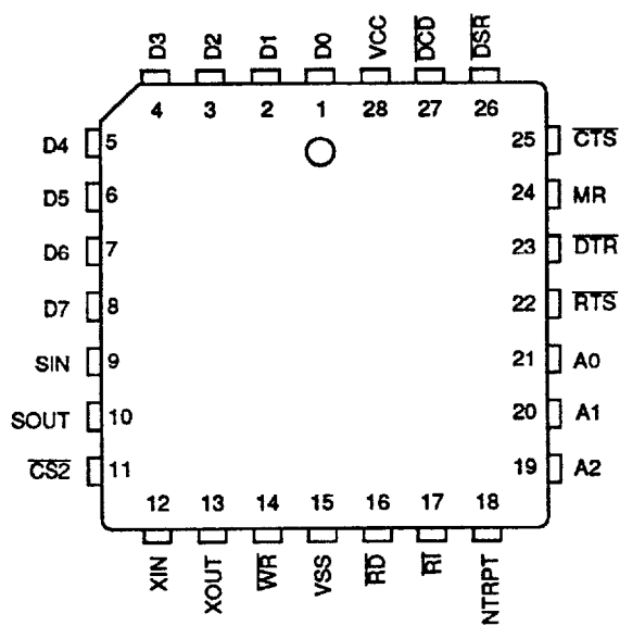
SSI 73M1550 UART 28-Pin PLCC
