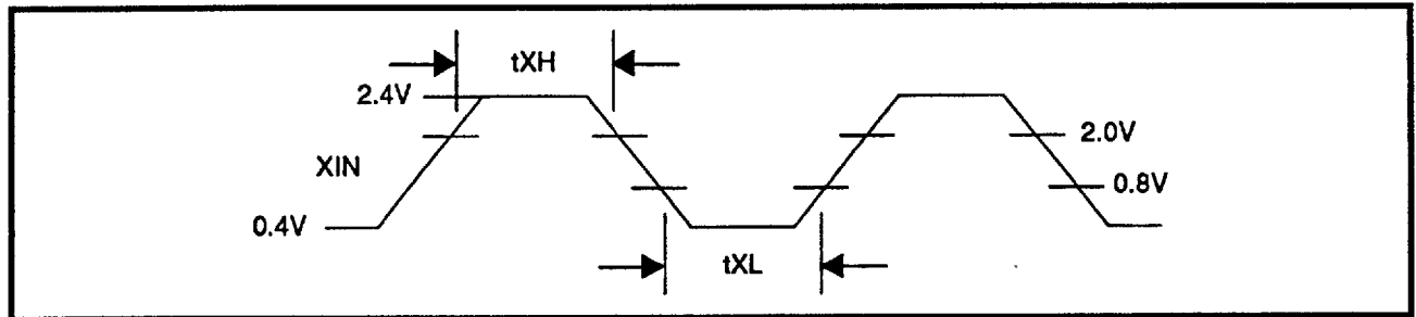
FIGURE 2: External Clock Input* (8 MHz Maximum)
