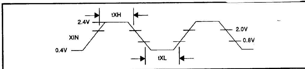
FIGURE 2: External Clock Input* (8 MHz Maximum)
