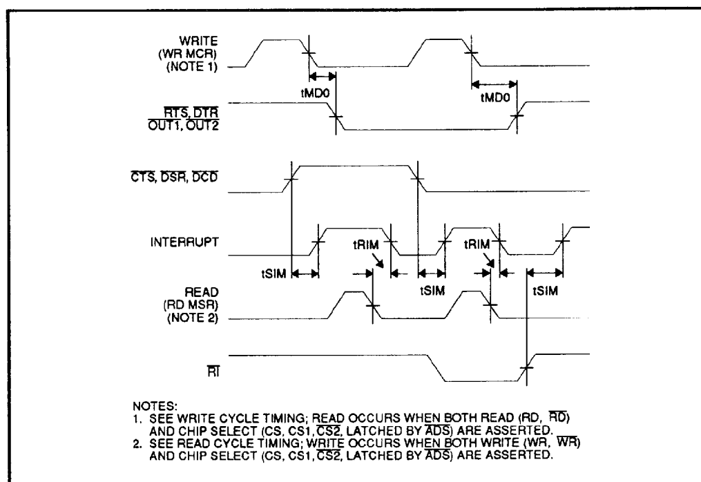
FIGURE 9: Modem Controls Timing
