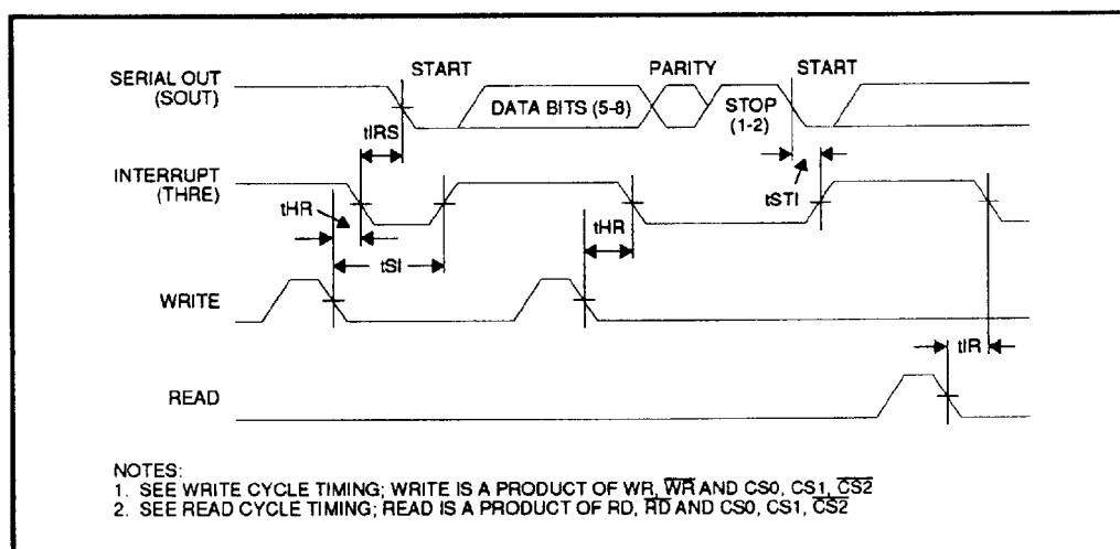
FIGURE 6: Transmitter Timing
