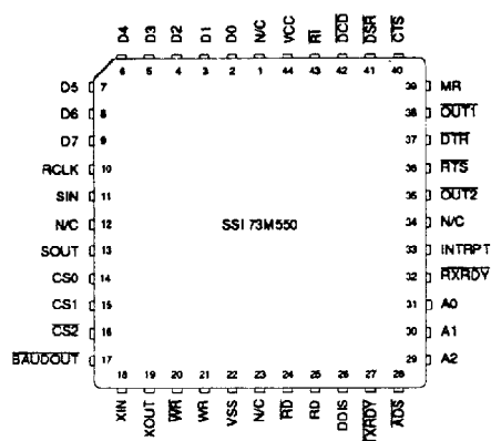
SSI 73M550/550F 44-Pin PLCC
