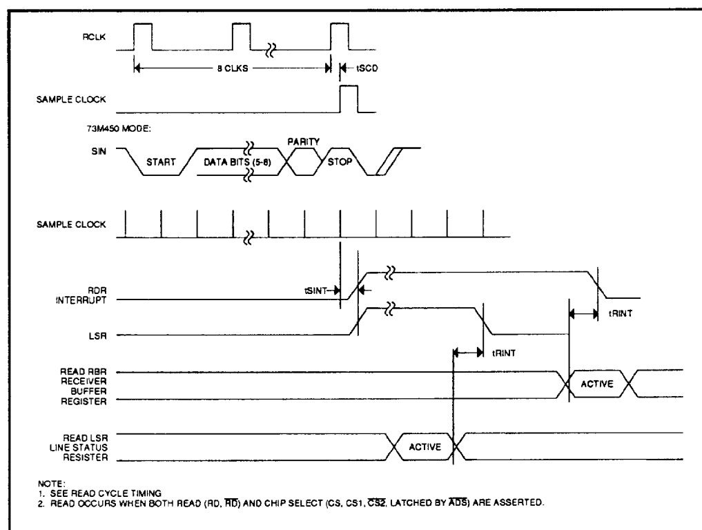
FIGURE 11: Receiver Timing
