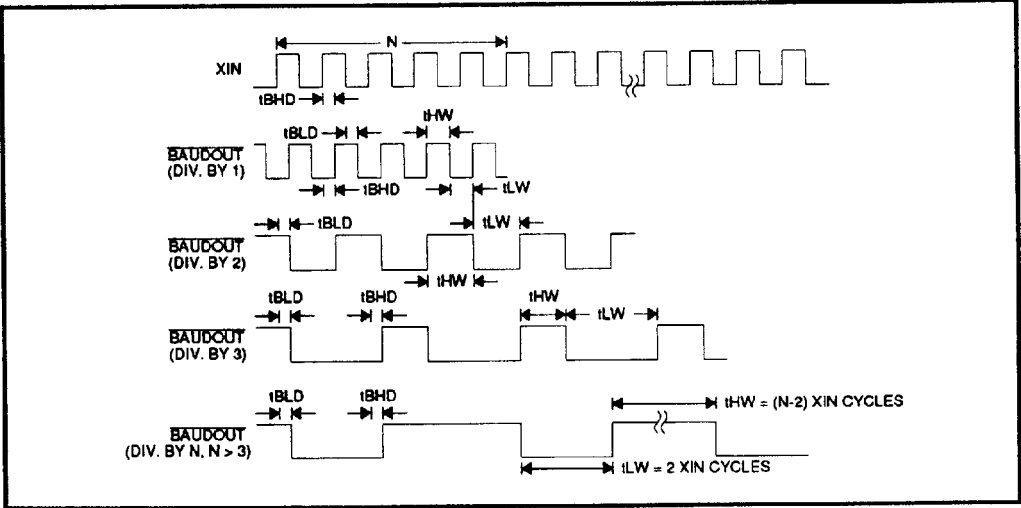
FIGURE 10: BAUDOUT Timing
