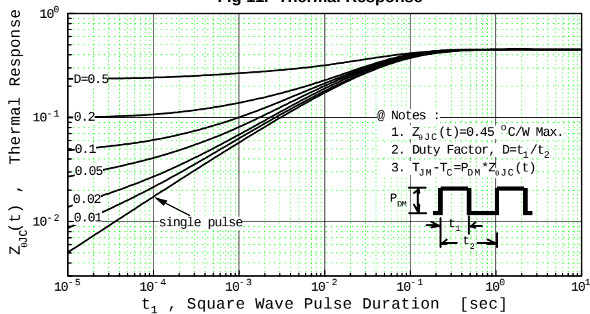
Fig 11. Thermal Response
