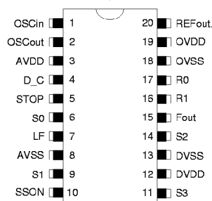
Figure 2. SM530, SSOP/TSSOP Package Pin Assignment
