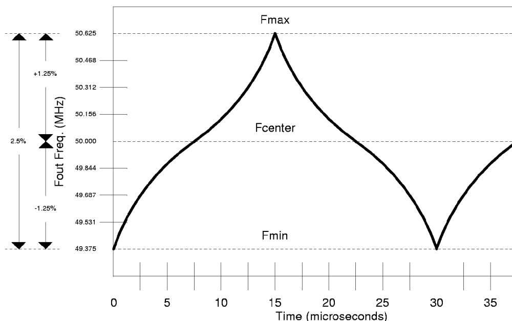
Figure 4. Modulation Profile
