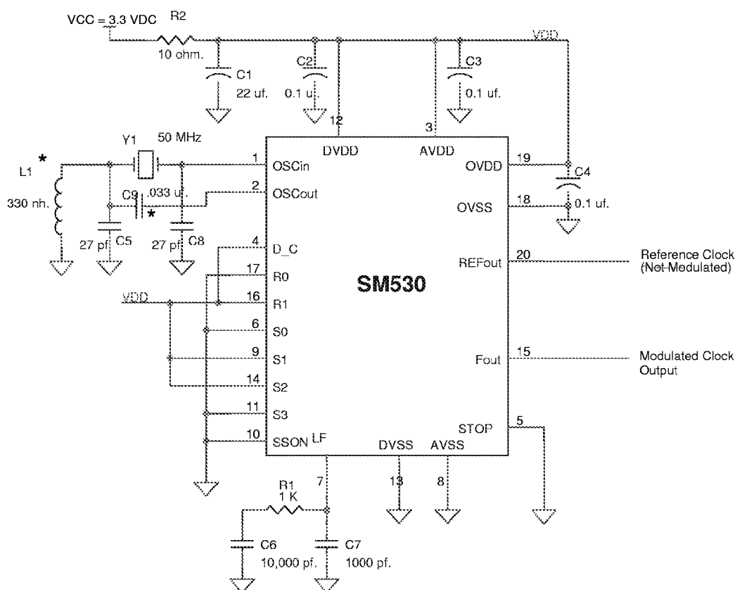
Figure 10. Application Schematic
