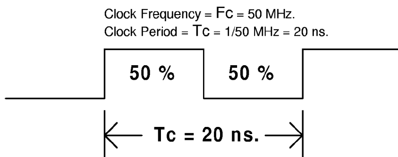
Figure 5. Unmodulated Clock
