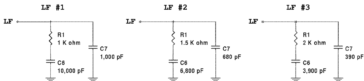
Figure 3. Recommended Loop Filter
