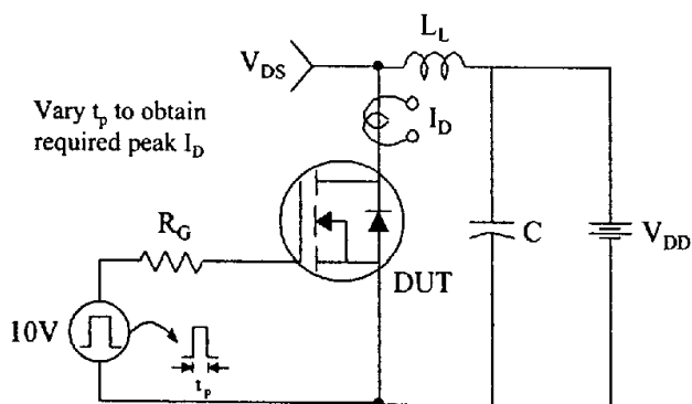
Fig 14. Unclamped Inductive Switching Test Circuit & Waveforms
