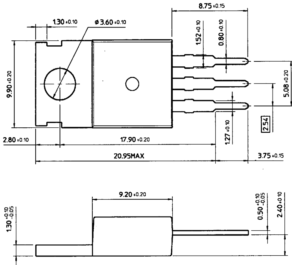
TO-220 (3)
