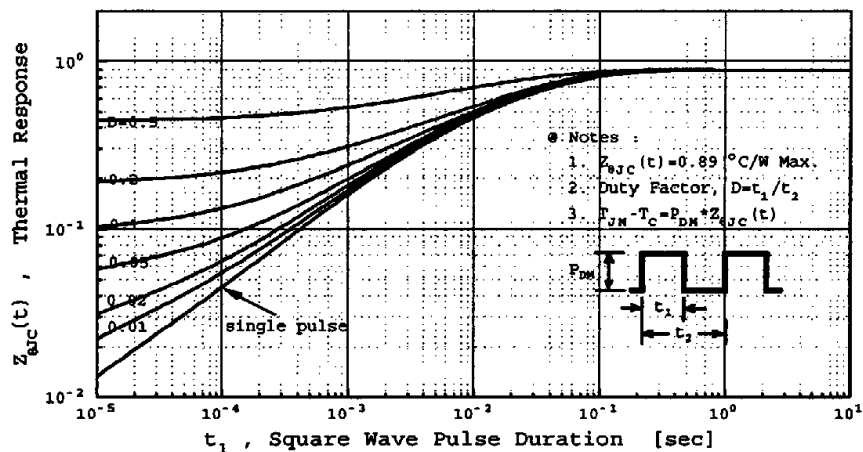
Fig 11. Thermal Response
