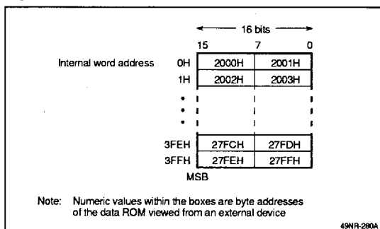
Figure 14. Data ROM
