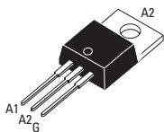
TO-220AB Non-Isolated (CHTB35)
