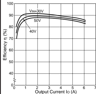
Efficiency Characteristics
