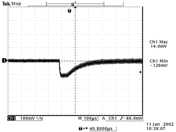
50% to 100% load transients at 3.3V input and Ta=25° C
