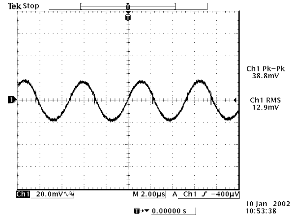
Ripple and noise at full load and 3.3Vdc input and Ta=25° C
