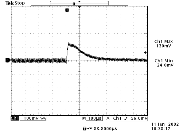
100% to 50% load transients at 3.3V input and Ta=25° C
