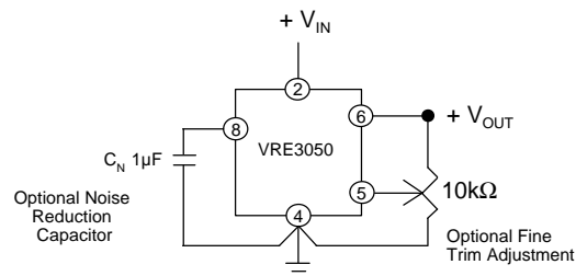
Figure 3 External Connections
