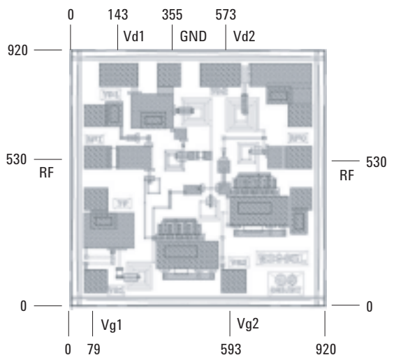
Figure 20. AMMC-5618 Bond pad locations (dimensions in microns)
