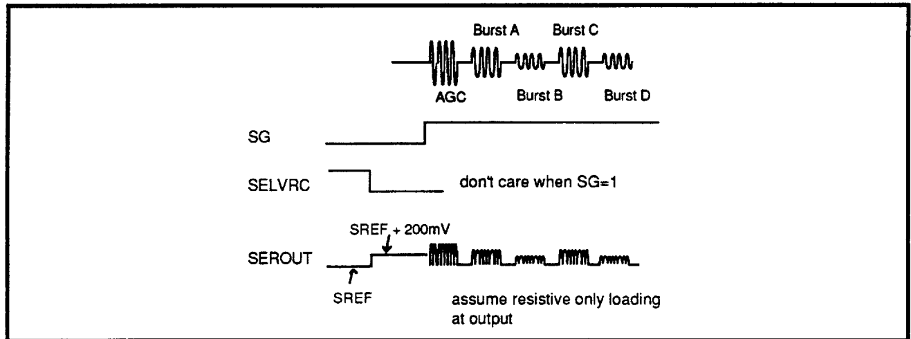
FIGURE 5: Sevo Function Diagram
