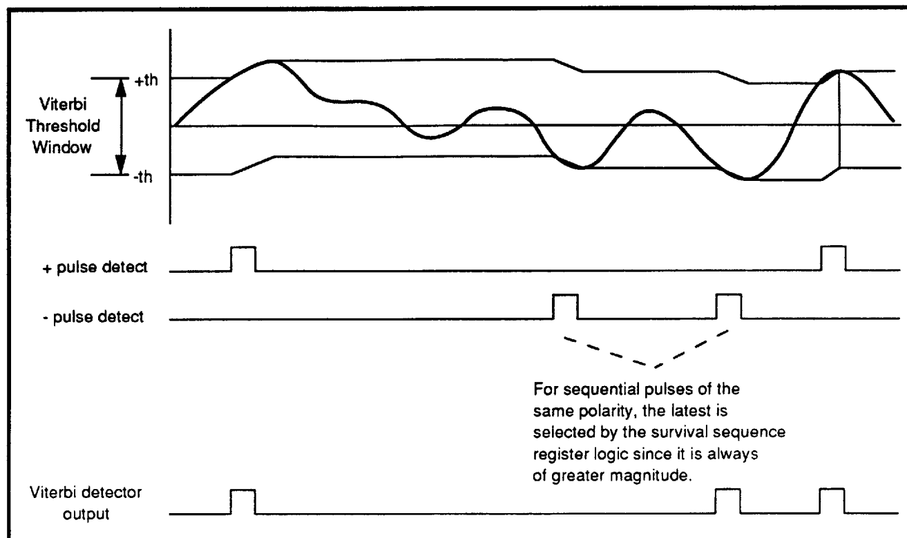
FIGURE 1: Viterbi Detection
