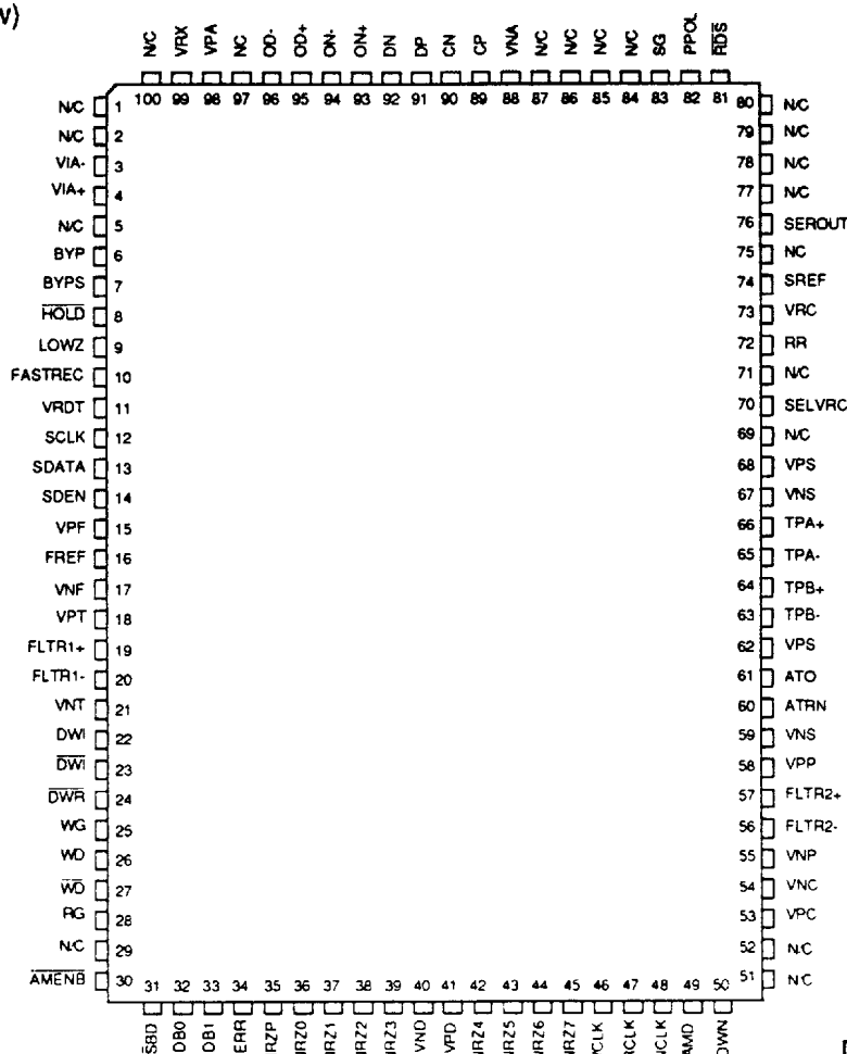
100-Lead QFP
