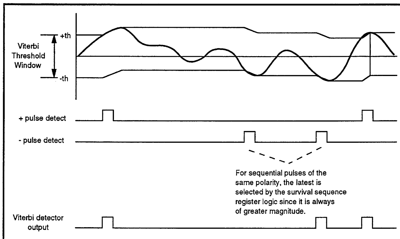
FIGURE 1: Viterbi Detection
