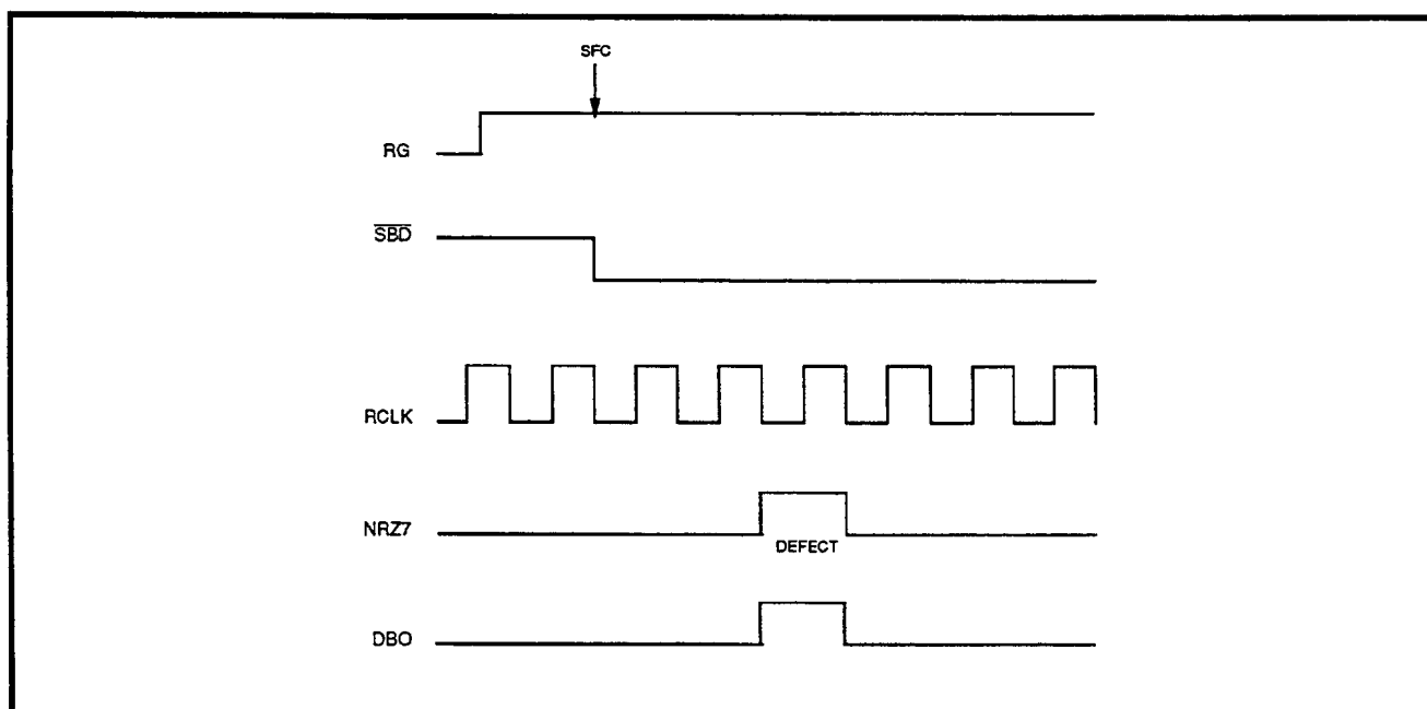
FIGURE 11: Surface Defect Scan Mode
