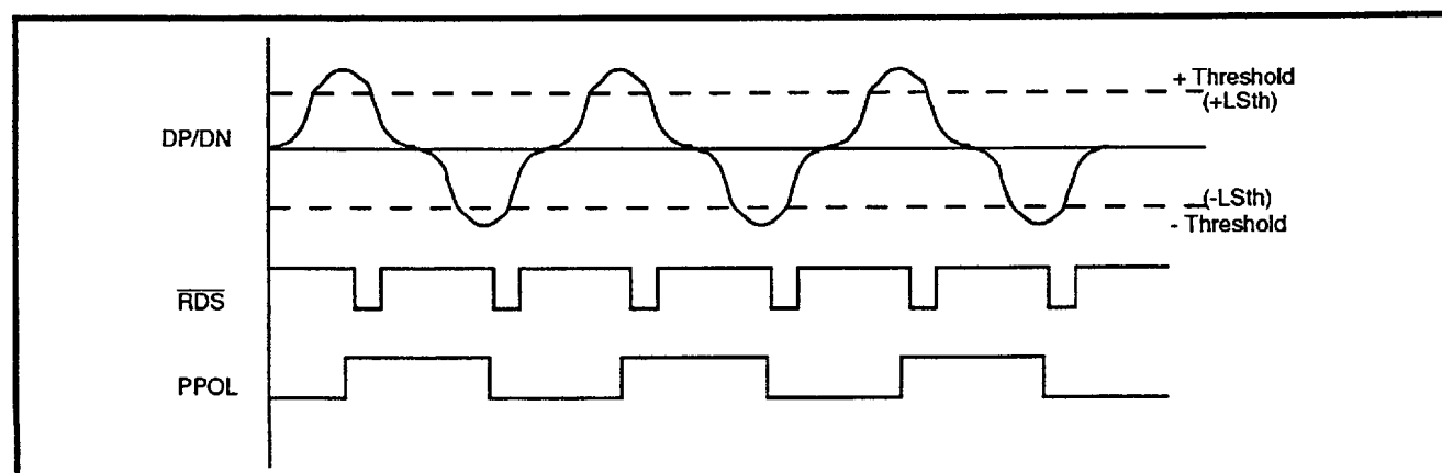
FIGURE 7: RDS and PPOL vs. DP/DN Relationship
