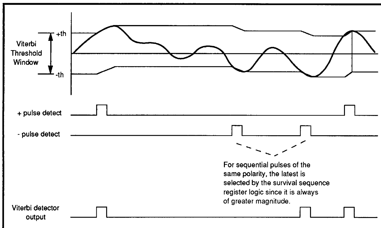
FIGURE 1: Viterbi Detection
