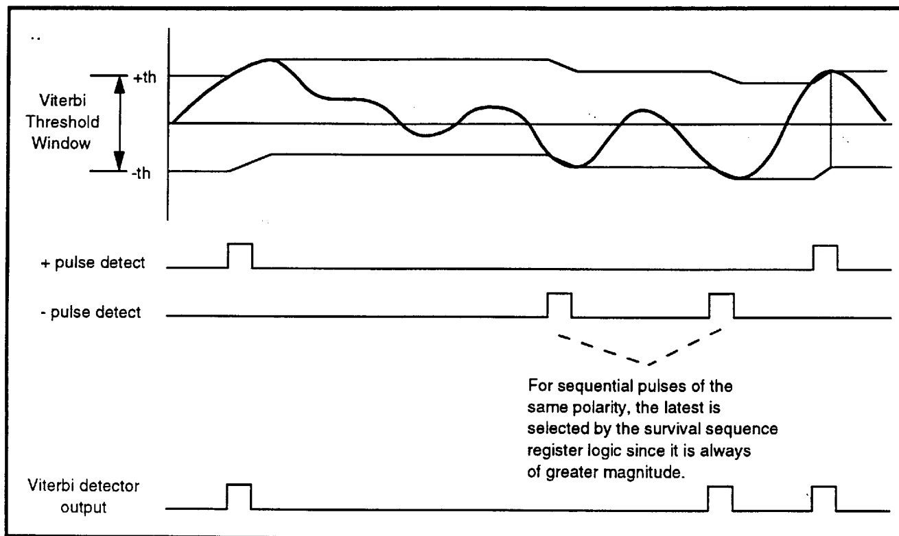
FIGURE 1: Viterbi Detection
