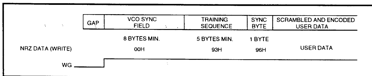
FIGURE 8: Hard Sector Write Sequence
