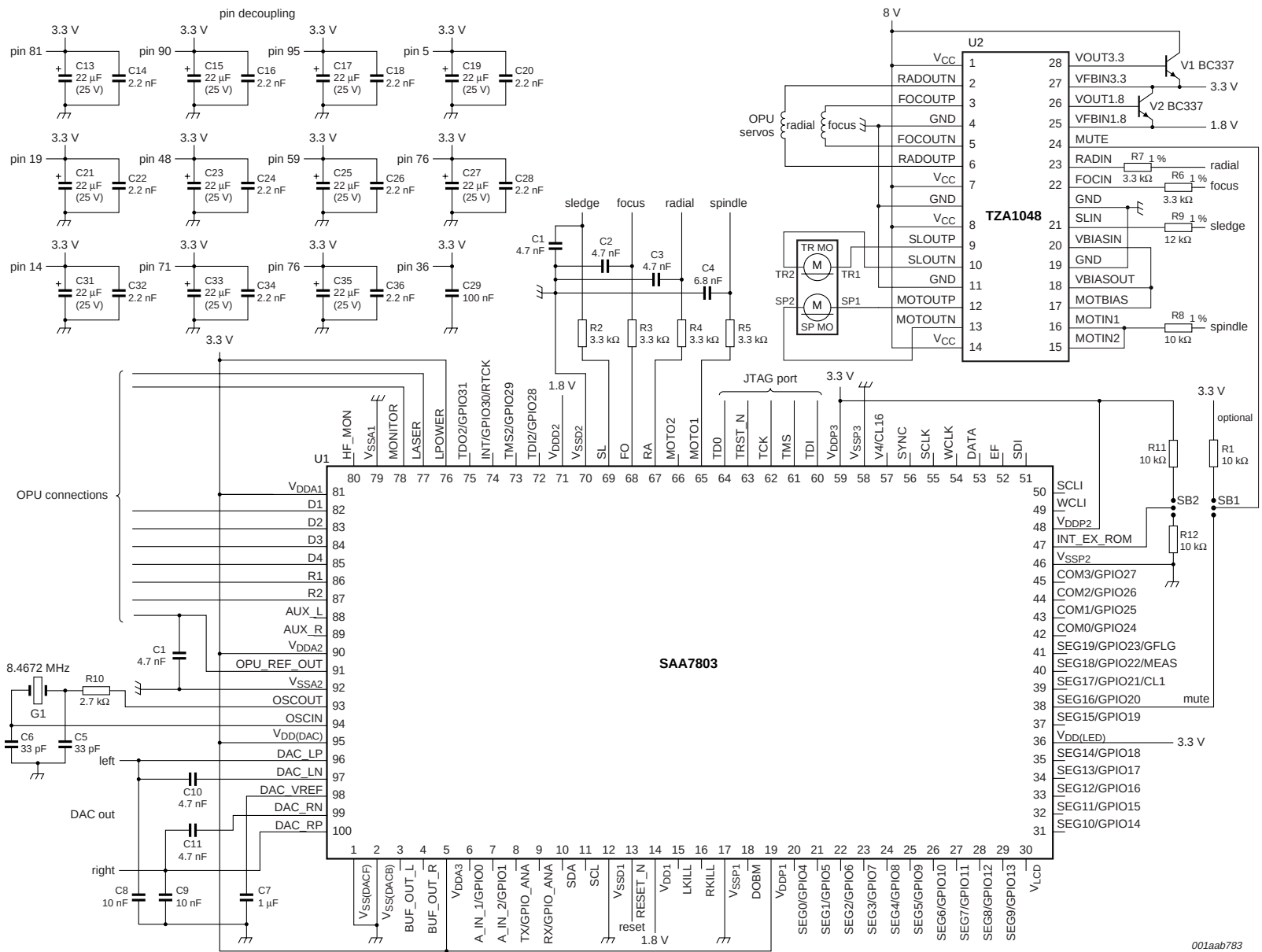
Fig 38. Typical application diagram
