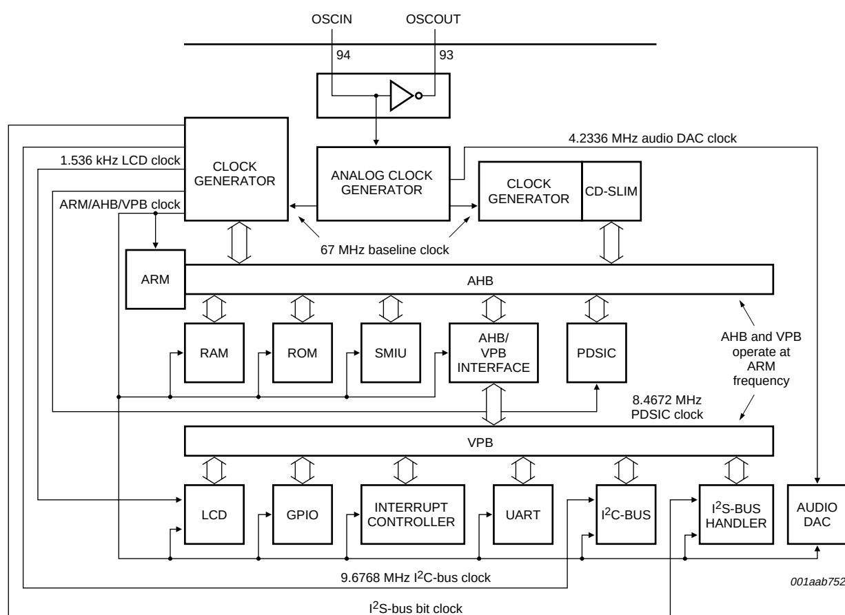
Fig 8. Clocking top level
