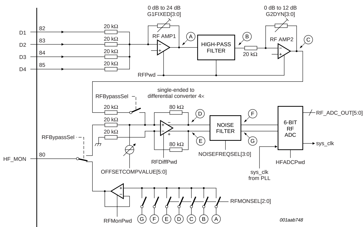
Fig 4. HF acquisition
