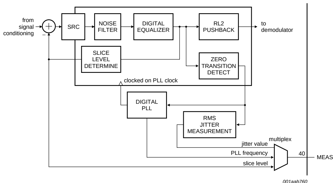
Fig 16. Bit detection
