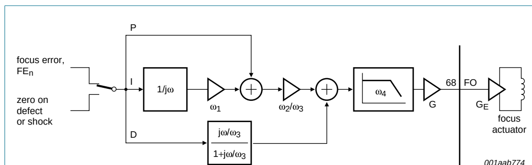
Fig 31. Functional diagram of focus PID system
