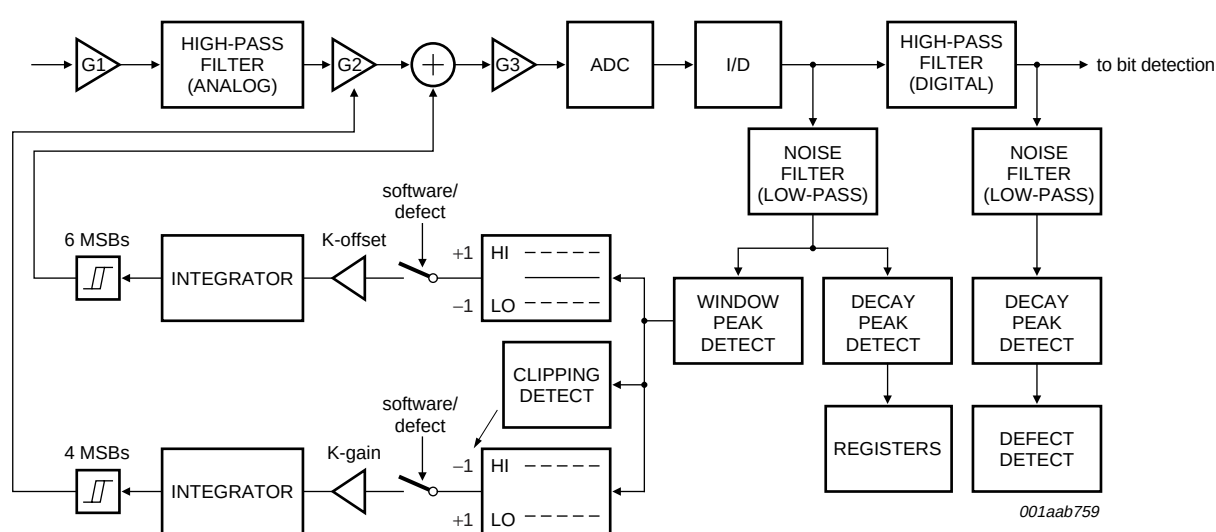
Fig 15. AGC and AOC loops
