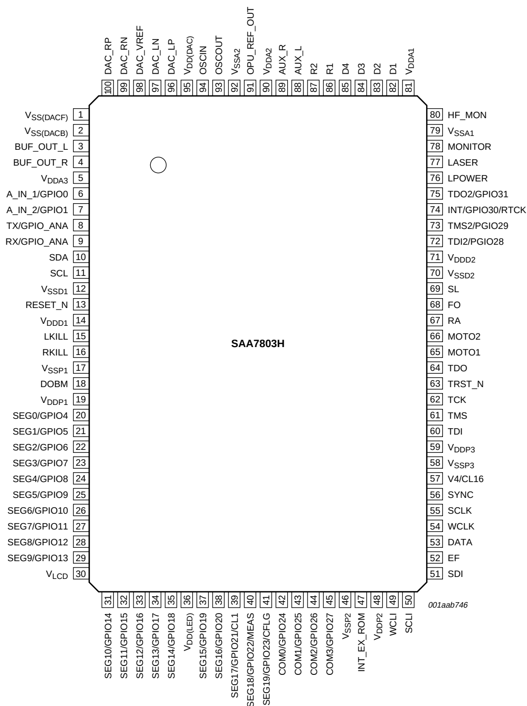
Fig 2. Pin configuration
