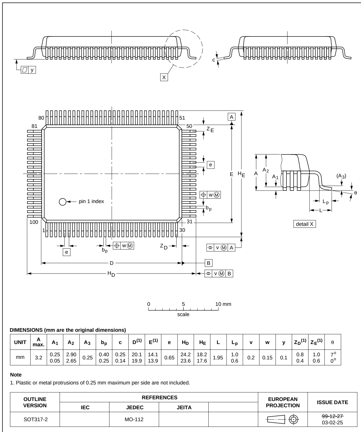
Fig 39. Package outline SOT317-2 (QFP100)
