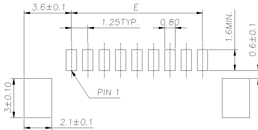
PCB LAYOUT FOR SURFACE MOUNTING
