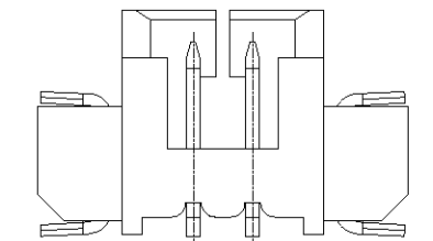
2 PIN
