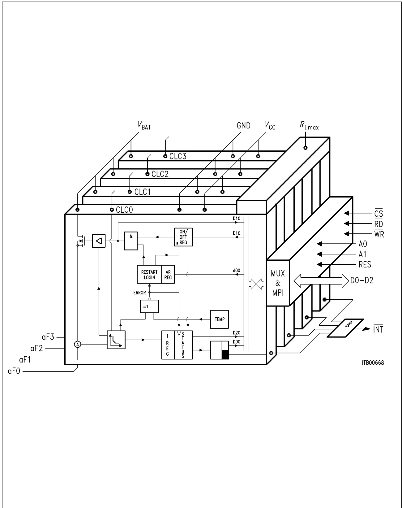
Figure 2 IEPC Architecture
