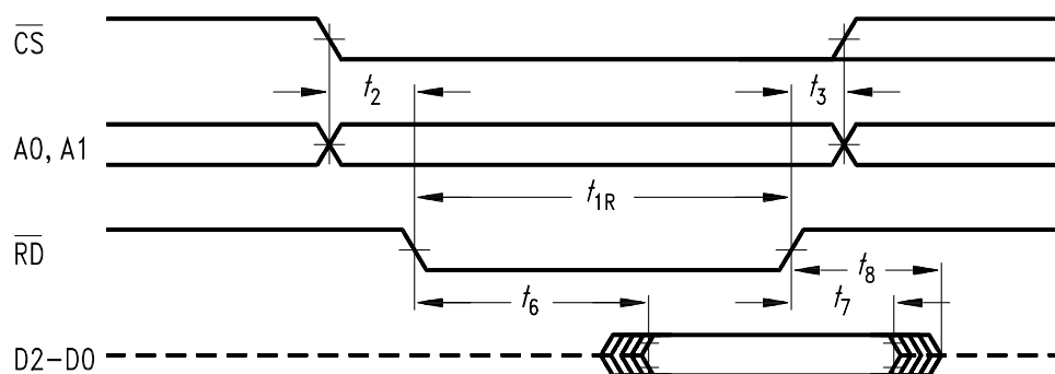
Read Timing
