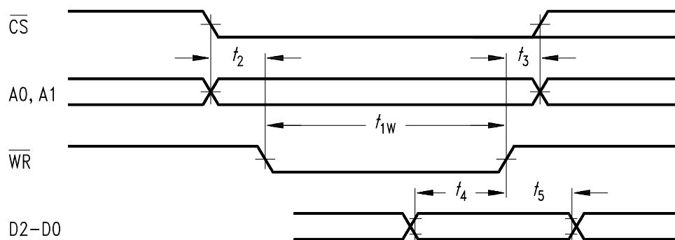
Write Timing
