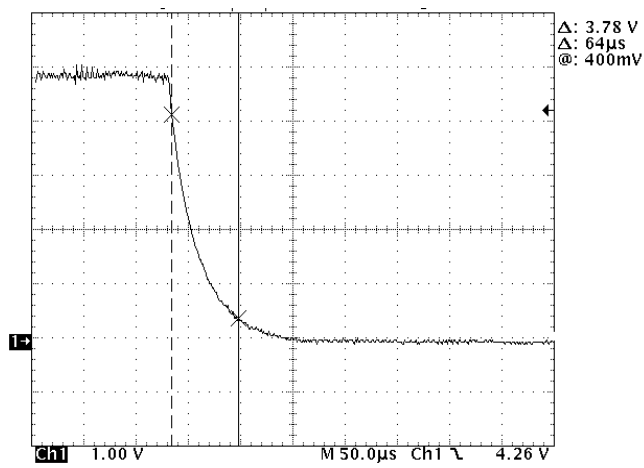
Typical CRD_VCC Fall Time @ Cout = 10 μF, V = 5.0 V
