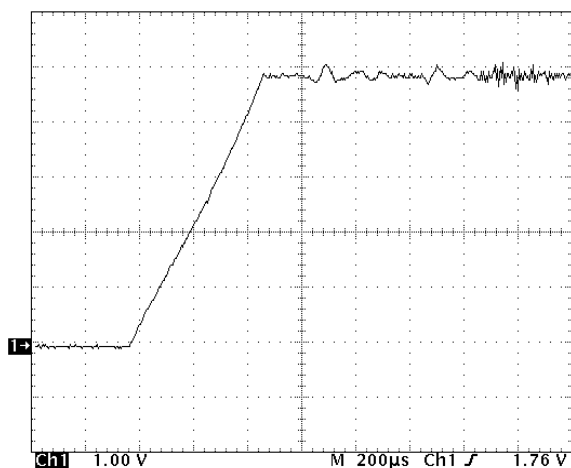
Typical CRD_VCC Rise Time @ Cout = 10 μF, V = 5.0 V
