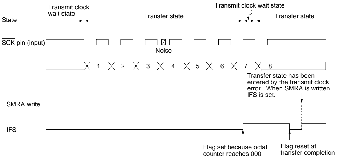
Figure 73 Transmit Clock Error Detection
