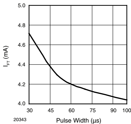
Figure 9. Trigger Current vs. Pulse Width
