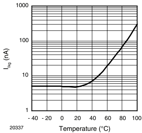
20337 Figure 3. Off-State Leakage Current vs. Temperature
