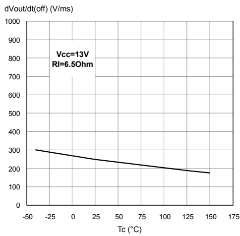
Figure 24. Turn-off Voltage Slope
