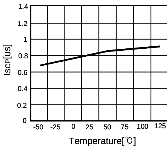
8. Temperature vs. T SCP
