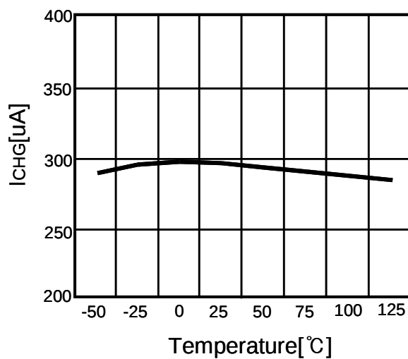
6. Temperature vs. I CHG
