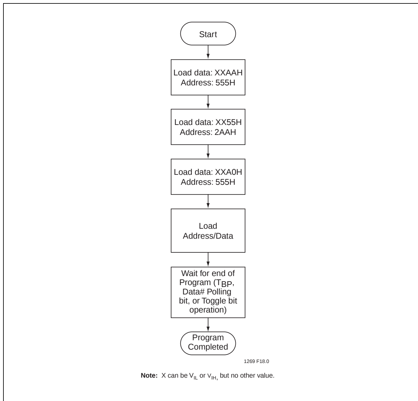
FIGURE 18: PROGRAM ALGORITHM
