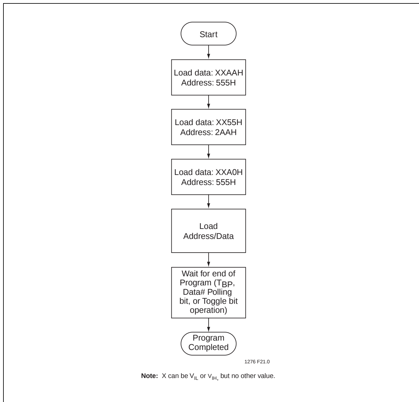
FIGURE 21: PROGRAM ALGORITHM
