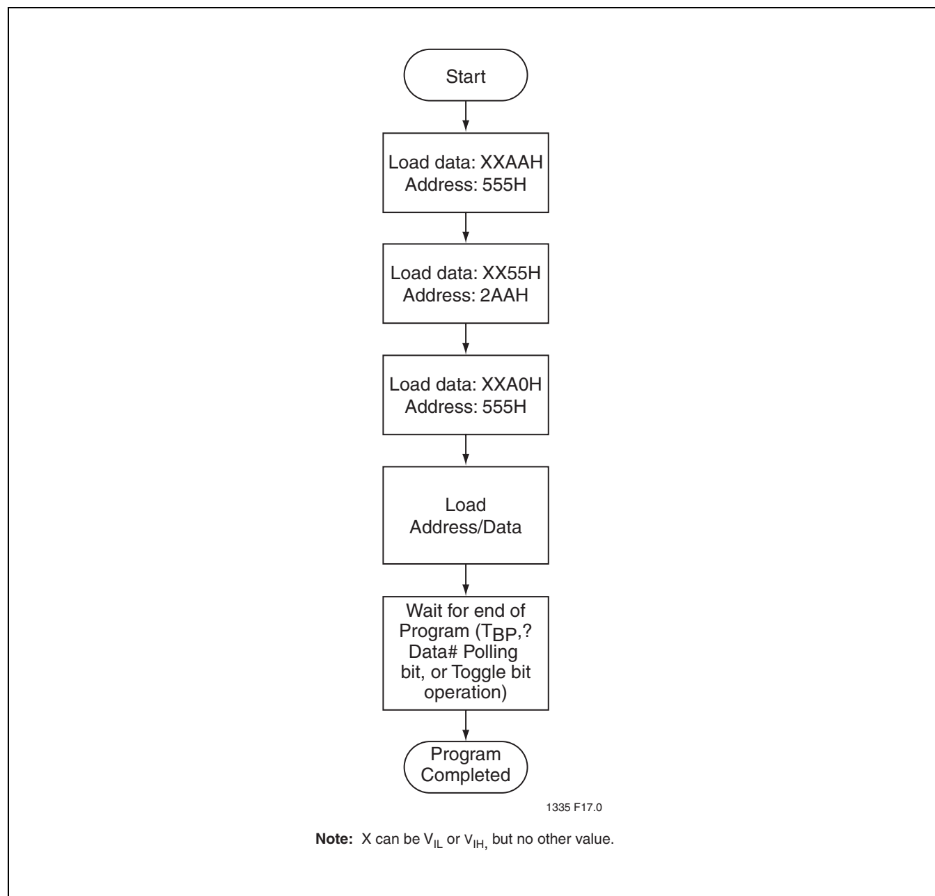
FIGURE 22: Program Algorithm
