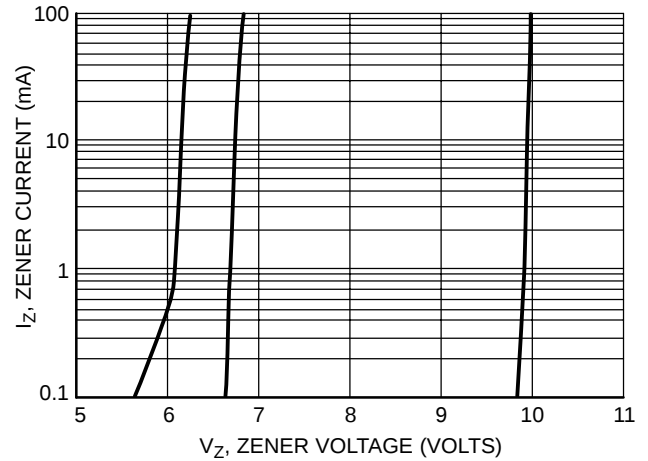
Figure 2. V_Z to 10 Volts
